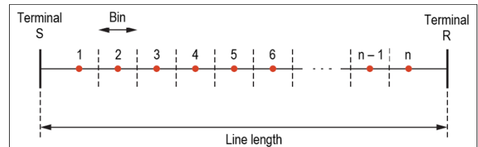
Fig. 9. The LIMO function divides the line into bins and counts the number of fault events located in each bin.
