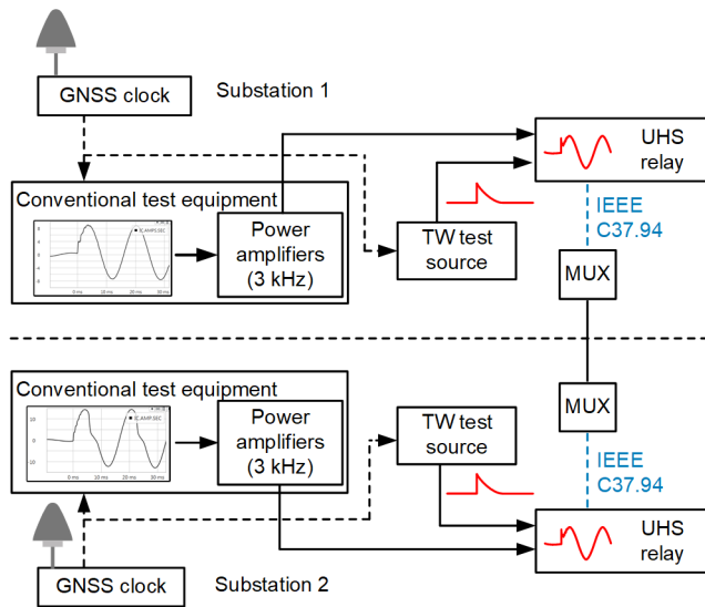
Fig. 13. SAT setup.
