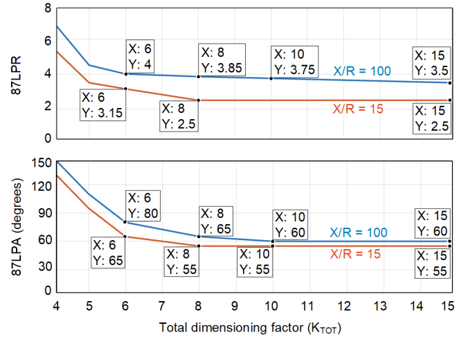
Fig. 8. 87AP blocking radius and angle requirements to accommodate CT saturation for systems up to different X/R ratios
