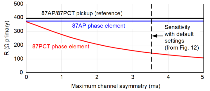
Fig. 13. Sensitivity comparison of 87AP and 87PCT phase element with equivalent settings for different levels of channel asymmetry
