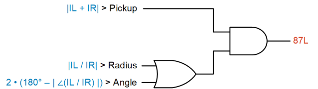
Fig. 2. Simplified logic for the 87L element using the alpha-plane principle
