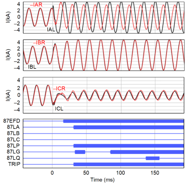
Fig. 11. Dependable operation of 87L elements despite 87EFD assertion
