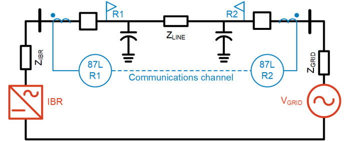
Fig. 1. Circuit relevant for 87L element
