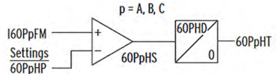
Fig. 4. High-set (conventional) split-phase element
