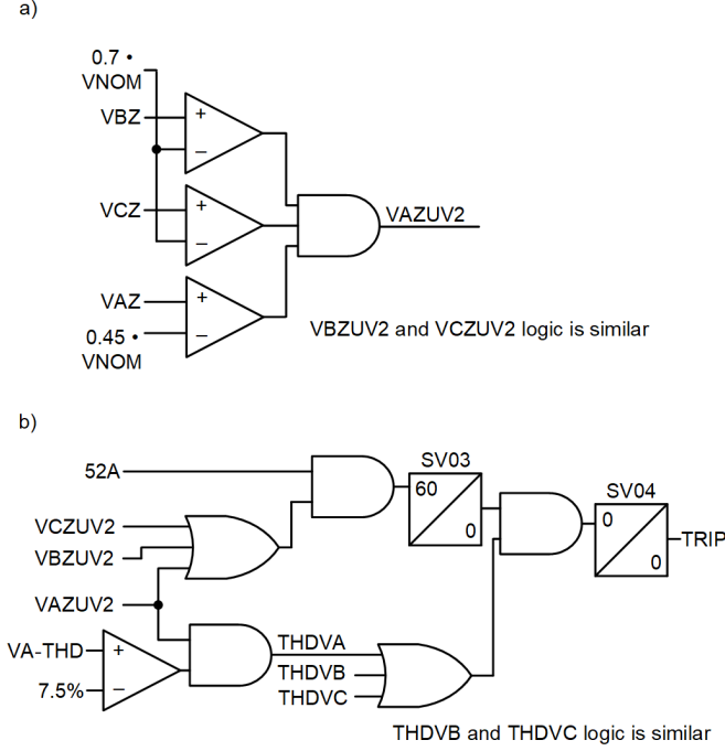
Fig. 9. (a) VZ Undervoltage Securing Logic for an Open-Phase Condition on the A-Phase (b) V-THD OPD Scheme
