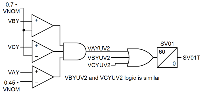
Fig. 7. VY Undervoltage Securing Logic for an Open-Phase Condition on the A-Phase
