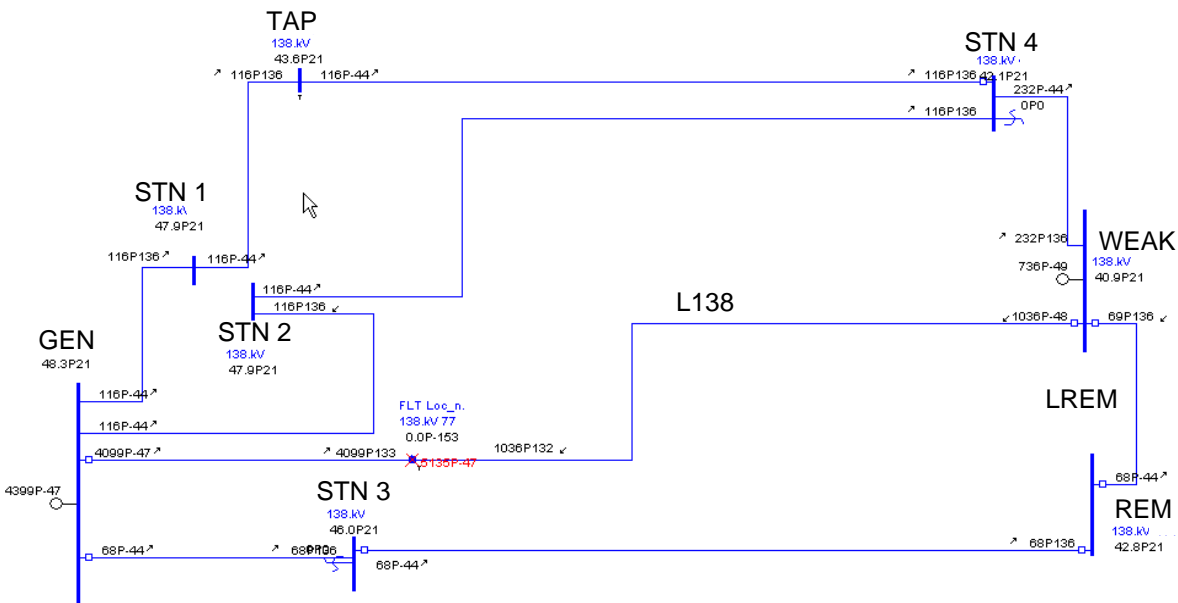
Figure 21 - Single line diagram of a faulted 138 kV line (L138) with simulation of the fault
