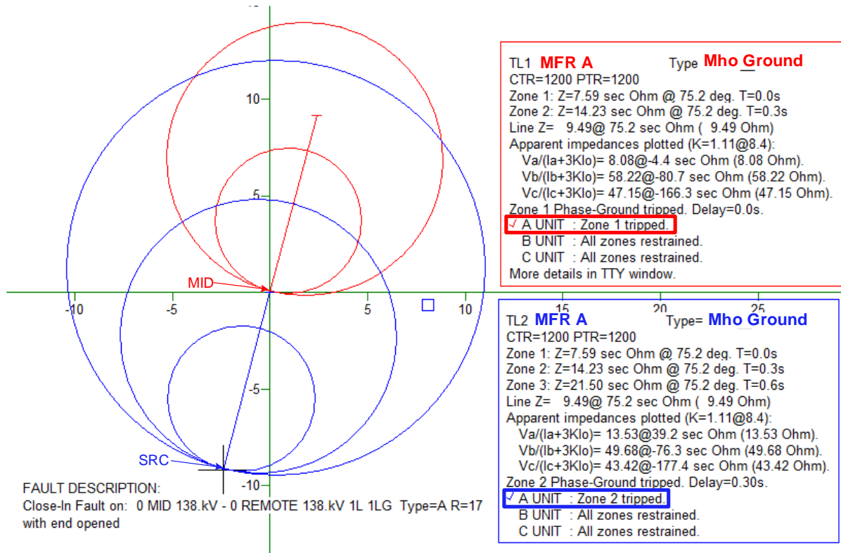
Figure 11 Backup relay coordinates well with Primary relay
