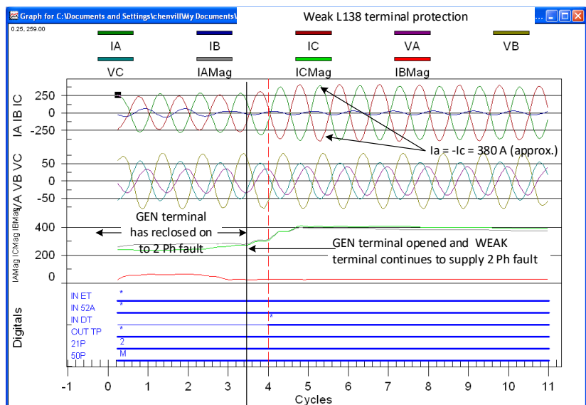
Figure 26 Record from WEAK Terminal after Automatic Reclose at GEN terminal of L138
