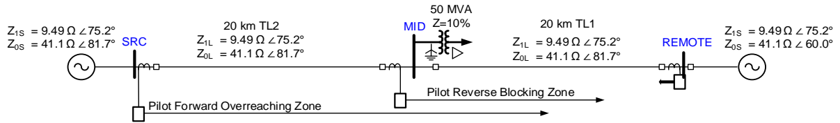
Figure 19 Example system showing relative reach of pilot reverse blocking zone with respect to pilot forward overreaching zone
