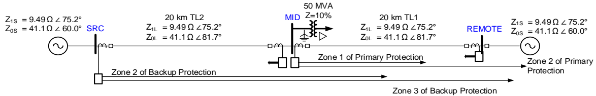
Figure 13 Example system with zero-sequence infeed at MID
