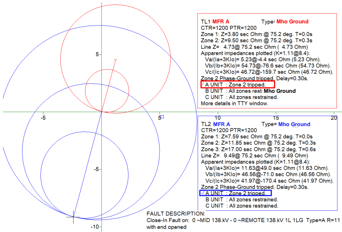
Figure 12 When primary relay reach is shortened, backup relay may operate simultaneously
