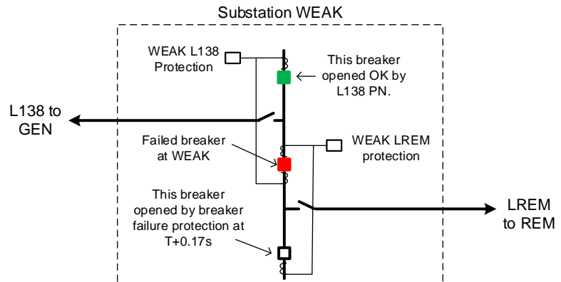
Figure 23 Single line diagram of part of Substation WEAK
