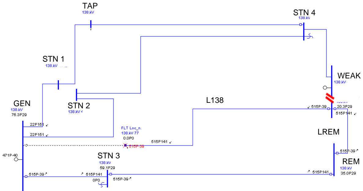
Figure 25 WEAK station reconfigured after breaker failure protection removes most infeed
