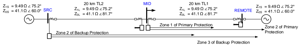
Figure 5 Example 138 kV system used to show coordination issues
