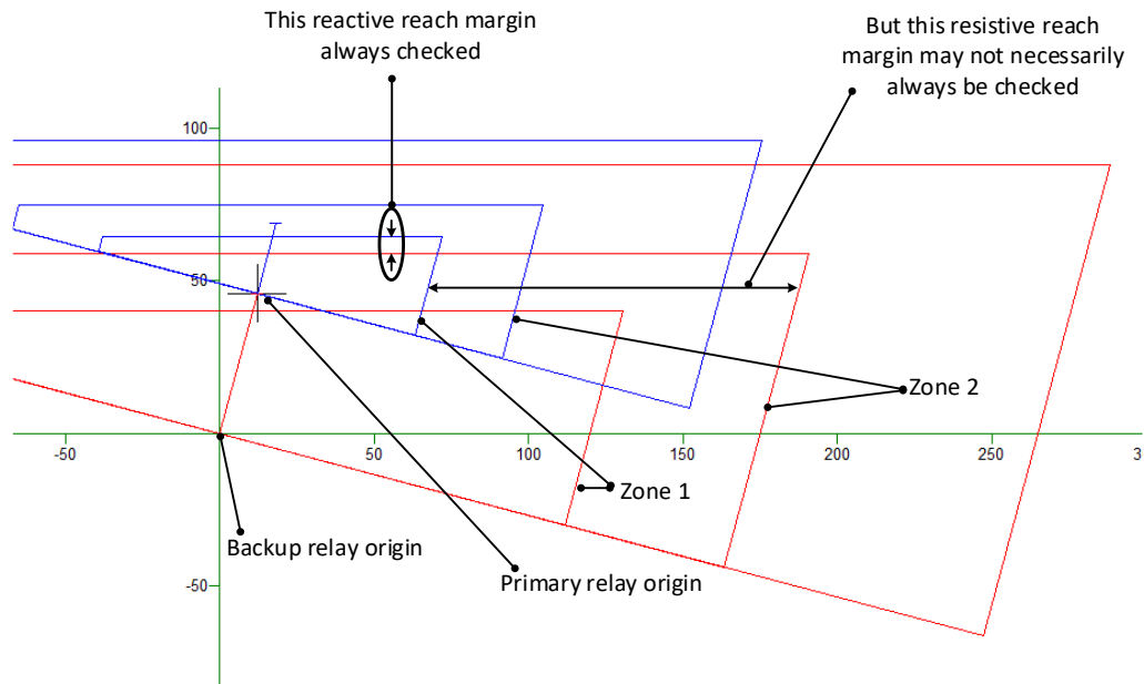
Figure 2 Coordination margins between a primary and backup relay pair
