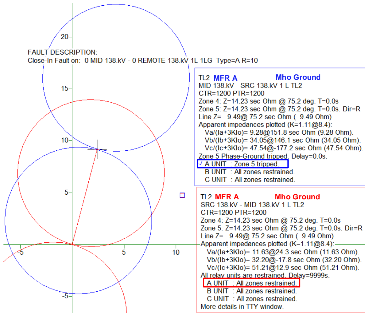
Figure 20 Pilot reverse blocking zone picks up and coordinates with forward overreaching zone
