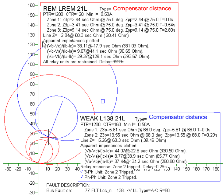
Figure 27 Responses of WEAK and BACKUP relays after GEN Terminal opens a second time
