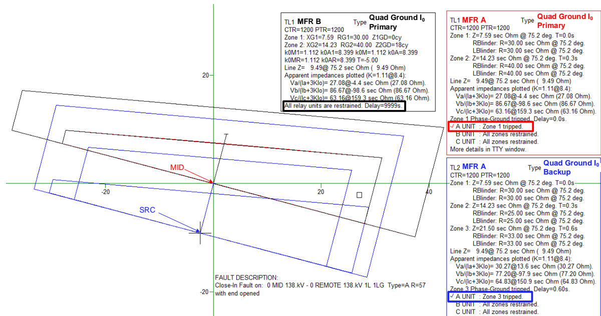
Figure 7 - Case 2, like Case 1, but with a different type of relay added to MID terminal of TL1
