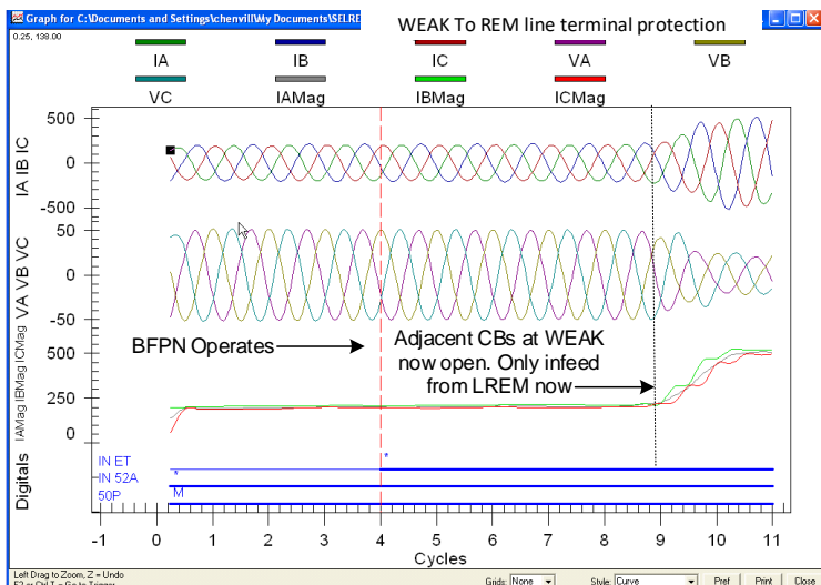
Figure 24 Infeed to WEAK Terminal from line LREM at T+0.17 s
