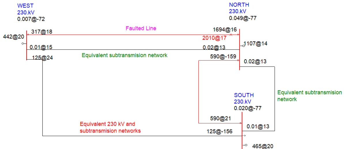
Figure 16 230 kV faulted network
