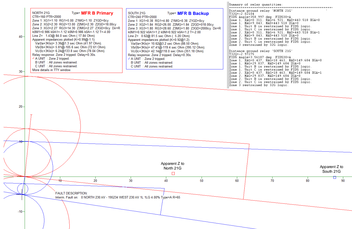
Figure 17 Reponses of primary and backup relays to the simulated fault
