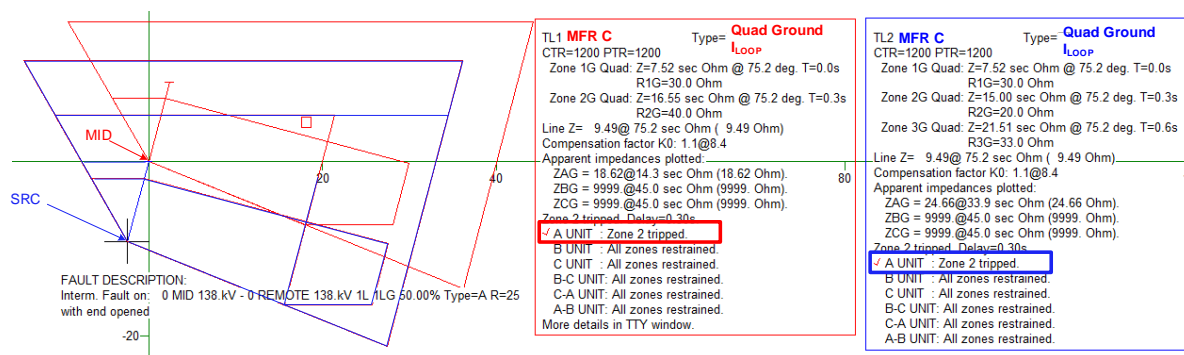
Figure 8 Zone 2 of the primary and backup relays operate simultaneously due to inconsistent tilt
