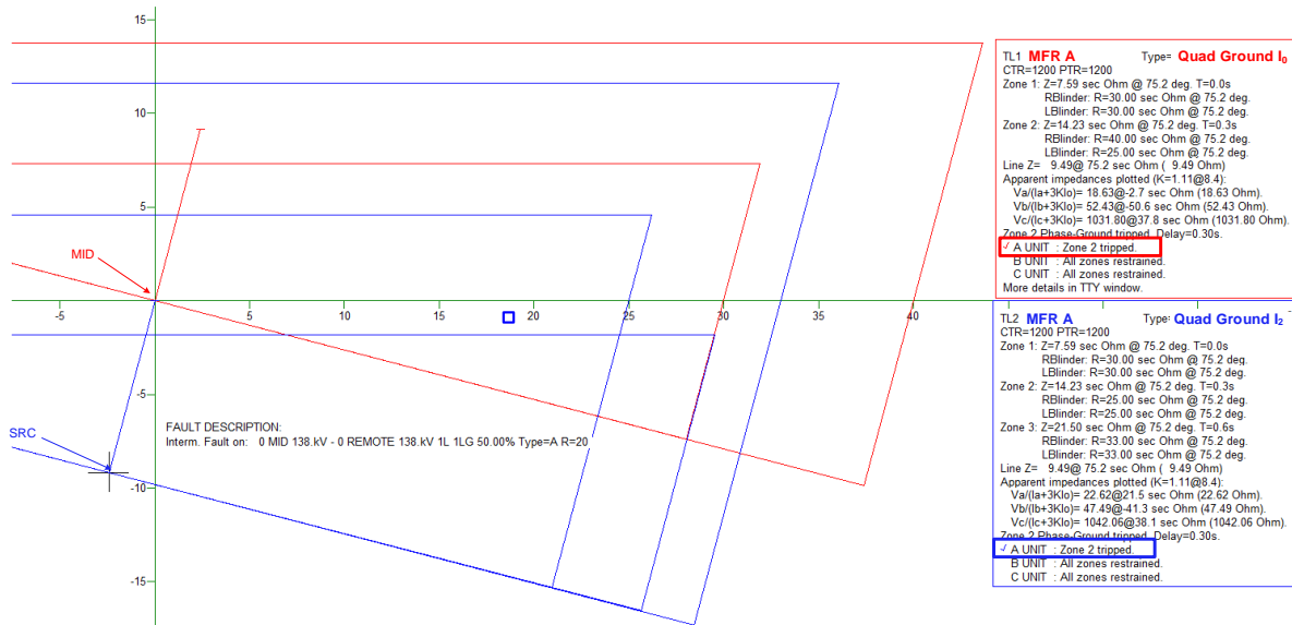
Figure 9 Zone 2 of the primary and backup relays operate at the same time due to use of different polarizing currents
