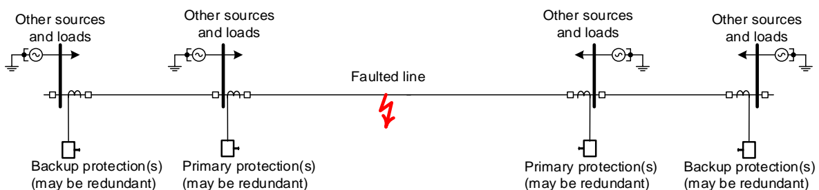
Figure 1 Example primary and backup protections
