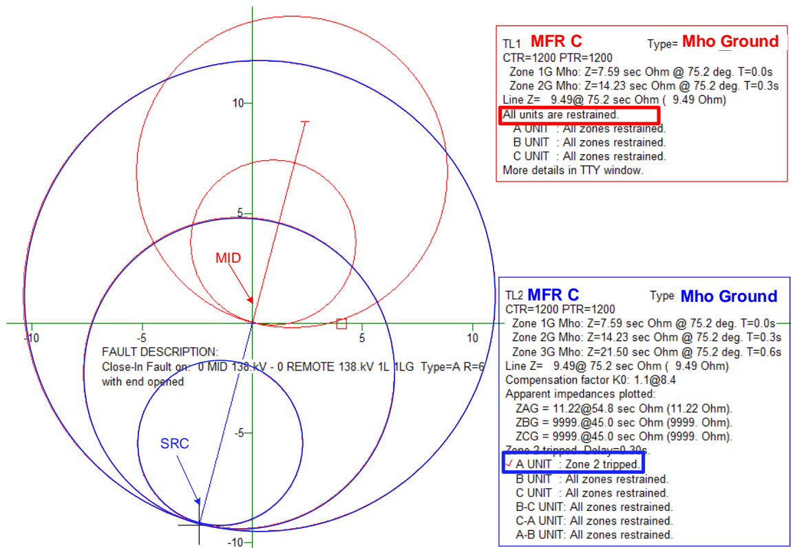
Figure 10 Primary relay does not trip whereas backup relay trips for a 6 Ω 1LG fault
