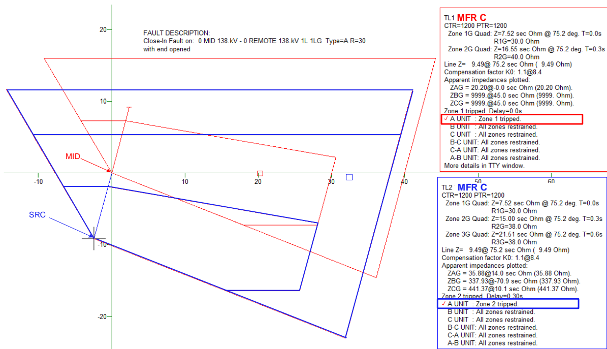
Figure 15 Coordination of self-polarized quadrilateral element considering infeed
