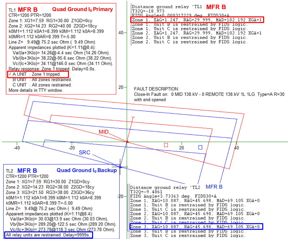
Figure 14 Coordination of ground quadrilateral element considering infeed
