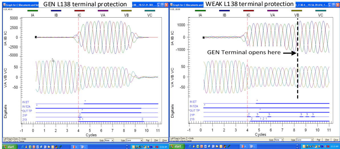
Figure 22 Recordings of initial three-phase fault from GEN (left) and WEAK (right) terminals
