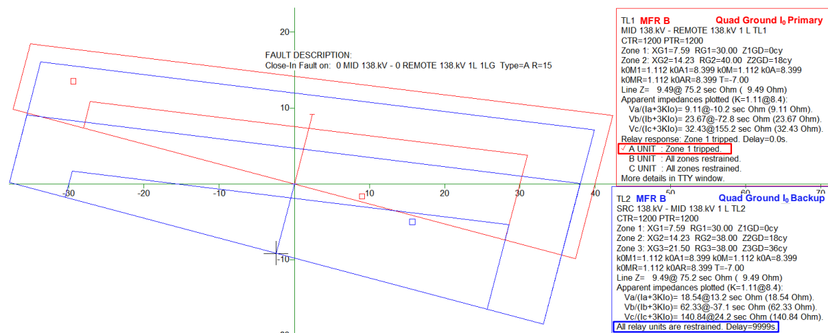
Figure 18 Zone 2 does not detect the fault and coordinates with Zone 1
