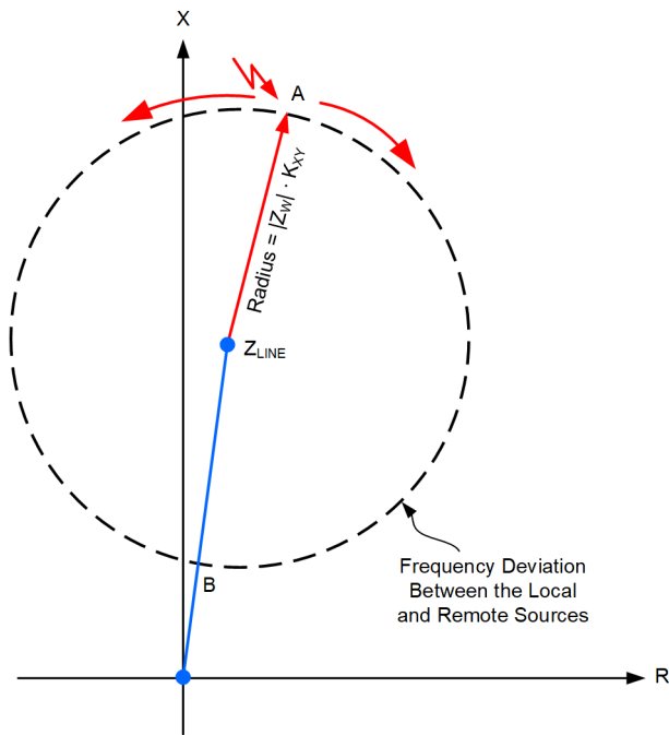
Fig. 4. Apparent impedance for the external fault in Fig. 2.
