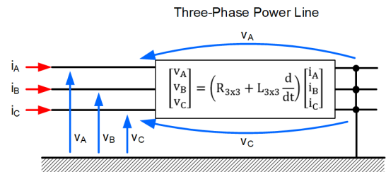
Fig. 5. Arbitrary current injected into a power line causes line voltages consistent with the R-L line parameters.
