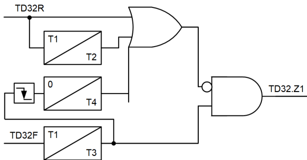
Fig. 20. TD32 directional logic for directionalizing and enabling the underreaching distance protection zone.
