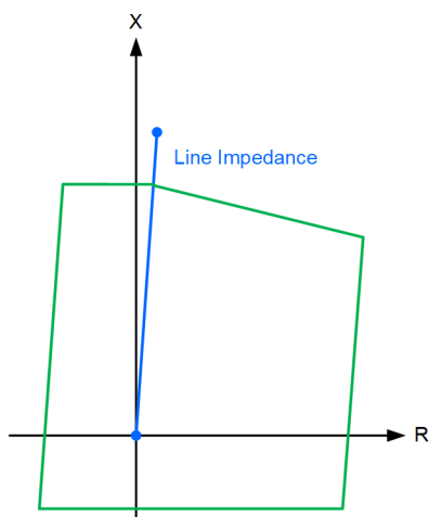
Fig. 10. Offset (nondirectional) apparent-impedance quadrilateral operating characteristic for underreaching applications with a reactance comparator security tilt.
