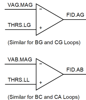
Fig. 21. Undervoltage faulted-loop selection logic with individual loop release.
