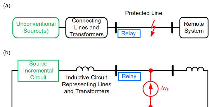
Fig. 15. Line fault in a system with an unconventional source (a) and the faulted-loop incremental-quantity equivalent circuit (b).
