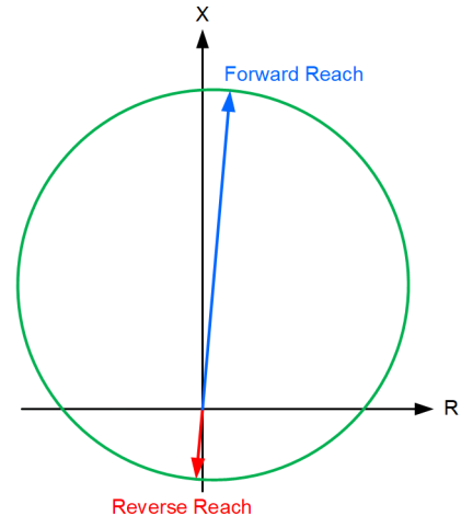
Fig. 8. Offset (nondirectional) apparent-impedance mho operating characteristic.
