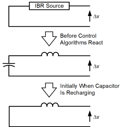
Fig. 16. Inverter-based source equivalent circuit during the first few milliseconds of a disturbance.
