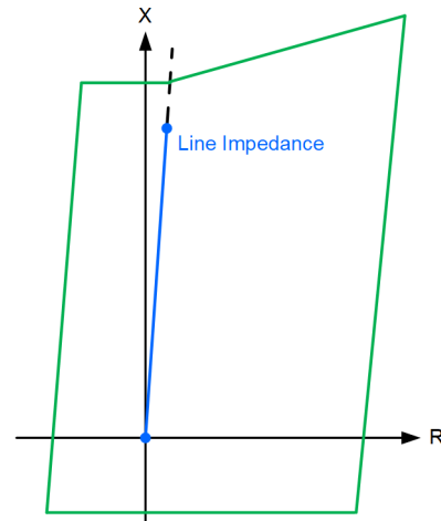
Fig. 11. Offset (nondirectional) apparent-impedance quadrilateral operating characteristic for overreaching applications with a reactance comparator dependability tilt.
