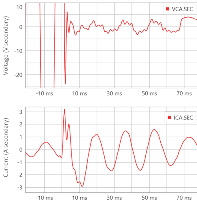
Fig. 27. Faulted-loop voltage and current for the case in Fig. 26.
