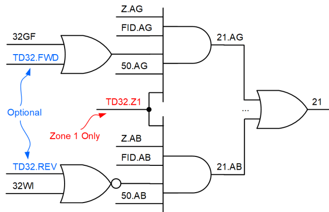
Fig. 23. Weak-infeed distance element logic.
