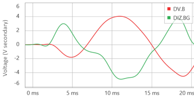
Fig. 17. Incremental voltage and incremental replica current in the BG loop for the case in Fig. 6 (the plotted voltage is scaled down to compare it with the current; the actual voltage is much higher).
