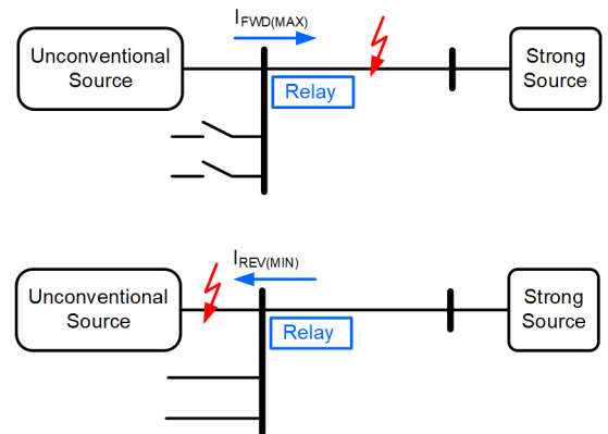
Fig. 13. 50WI overcurrent coordination principle.
