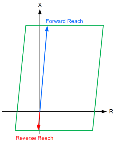
Fig. 9. Offset (nondirectional) apparent-impedance quadrilateral operating characteristic.
