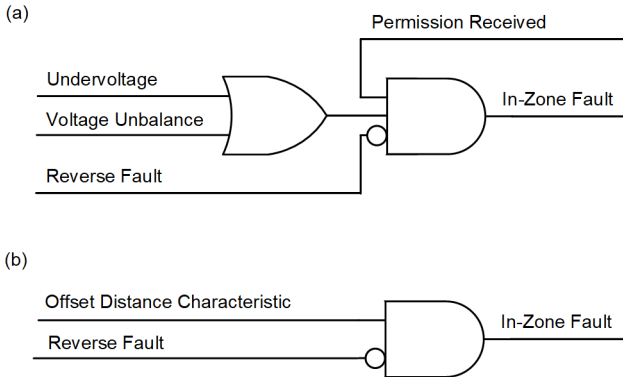
Fig. 12. Weak-infeed pilot logic (a) and weak-infeed directional distance logic (b).
