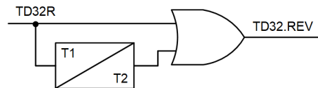
Fig. 18. Blocking TD32 directional logic for directionalizing overreaching distance protection zones.
