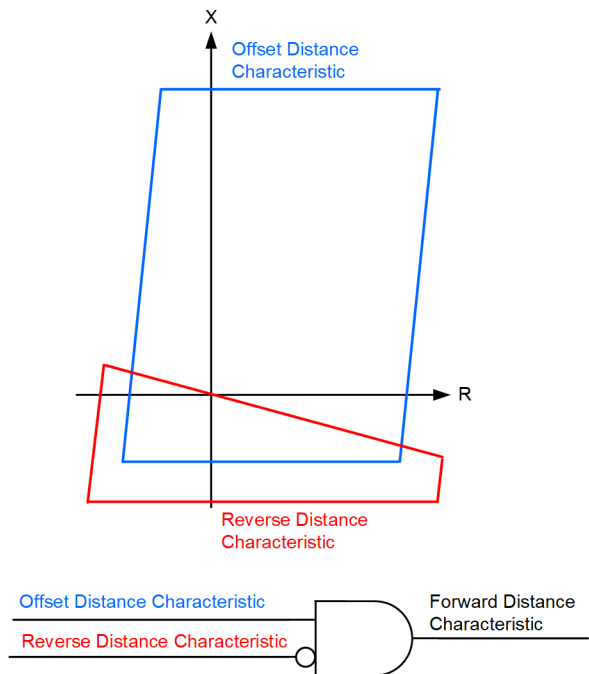
Fig. 14. Using a reverse-looking distance element to directionalize an offset distance characteristic.
