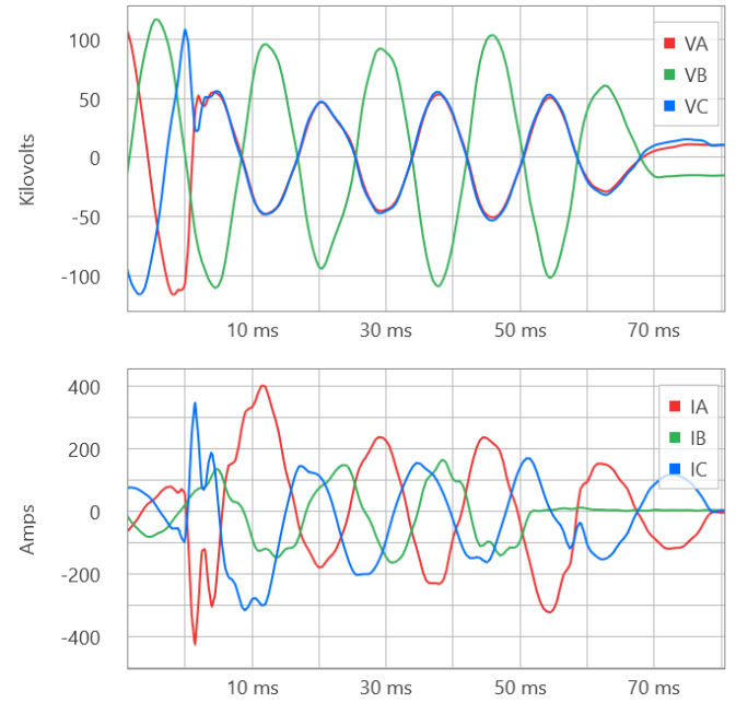
Fig. 26. Line relay voltages and currents supplied by an unconventional source for a phase fault.
