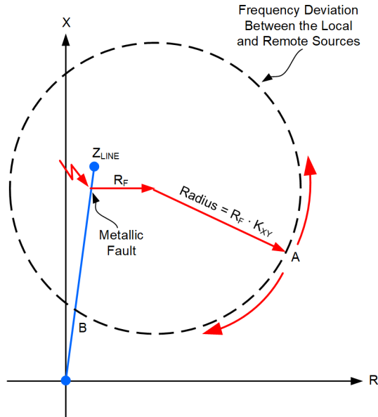
Fig. 3. Apparent impedance for the internal resistive fault in Fig. 1.
