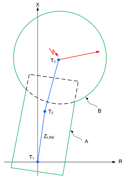
Fig. 24. A composite step distance element characteristic for applications intended to considerably overreach the remote line terminal.
