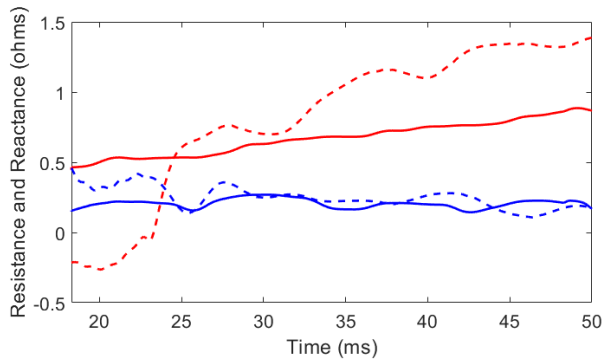
Fig. 28. The apparent resistance (red) and reactance (blue) in the CA loop for the case in Fig. 26: phasor-based approach (dashed lines) and time-domain wide-spectrum approach (solid lines).
