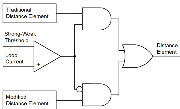
Fig. 25. Distance element application in systems with high short-circuit variability (either the unconventional source or the traditional system dominates the fault response).
