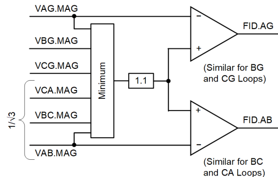
Fig. 22. Undervoltage faulted-loop selection logic with lowest-voltage single-loop release.
