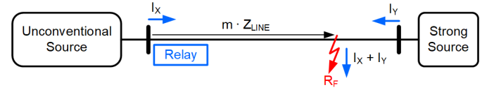
Fig. 1. Resistive fault near the remote terminal.
