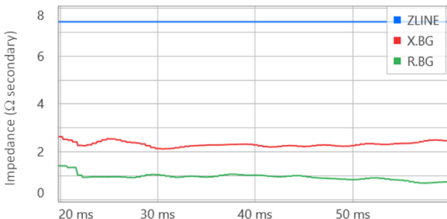
Fig. 7. Well-behaved apparent BG loop resistance and reactance for the heavily distorted waveforms in Fig. 6.
