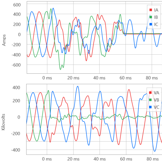
Fig. 6. Line voltages and currents for a BG fault in a system with an unconventional source behind the relay (field record).
