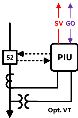
Figure 6: PIU concept
