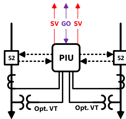
Figure 8: PIU shared between feeders
