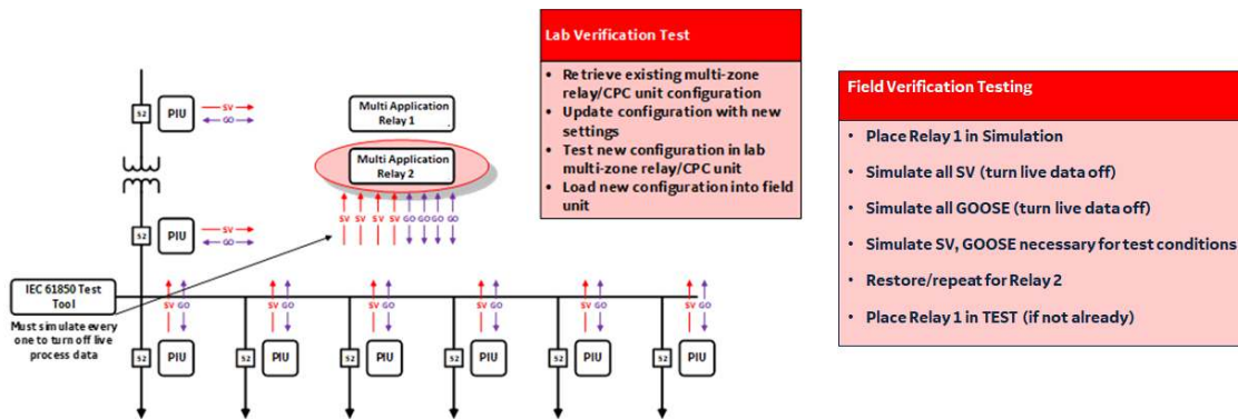
Figure 21: Testing a redundant multi applications relay substation
