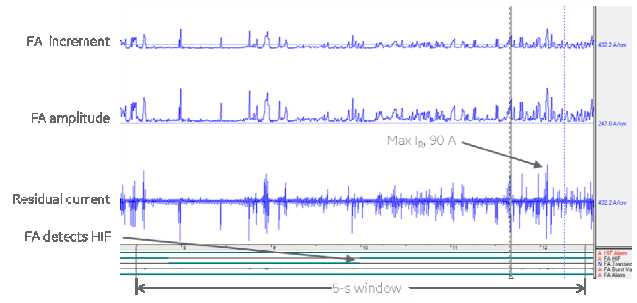
Fig. 7. Method P downed-conductor test result
