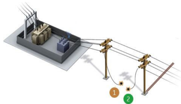
Fig. 2. Broken conductor
