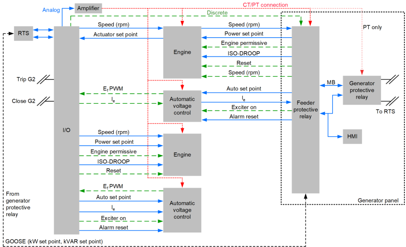
Fig. 11. Governor and exciter interface
