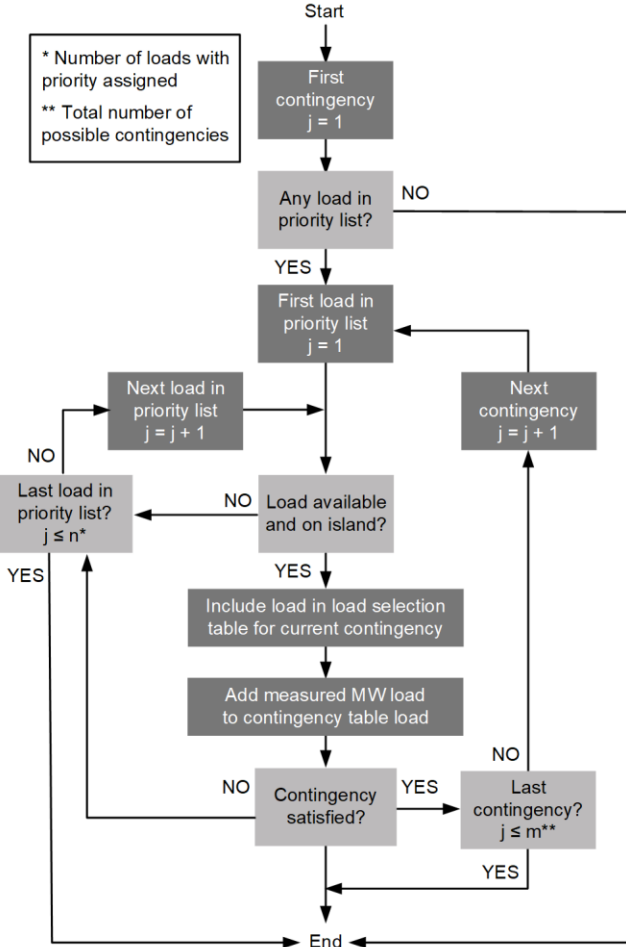
Fig. 4. Load selection flowchart
