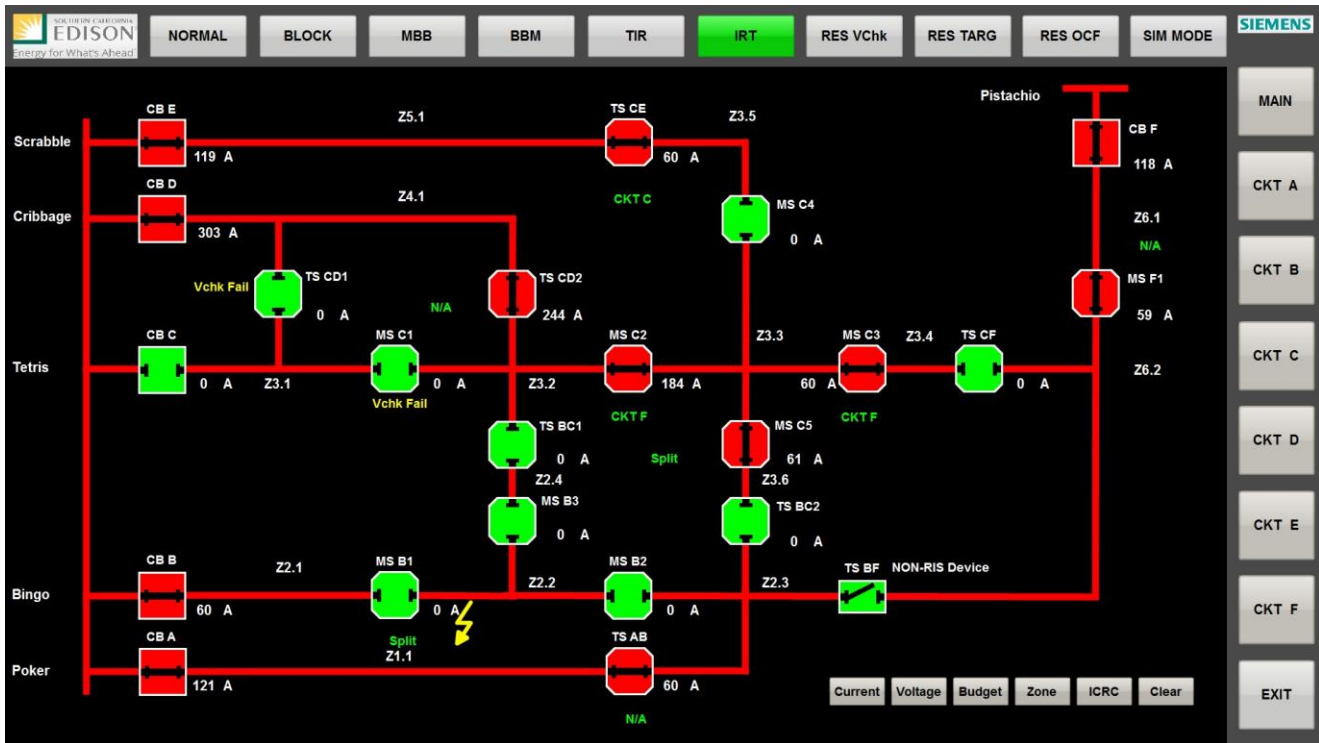
Fig.14. System response to evolving fault in Zone 2.2
