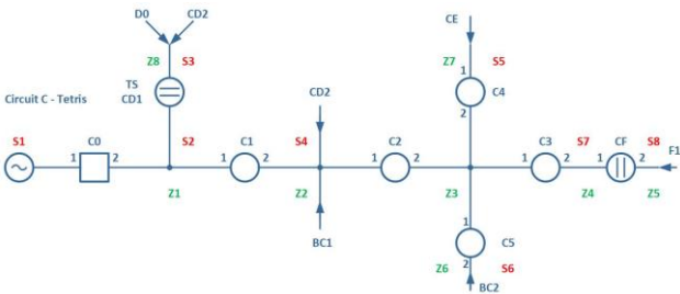
Fig. 5. RIS Circuit C
