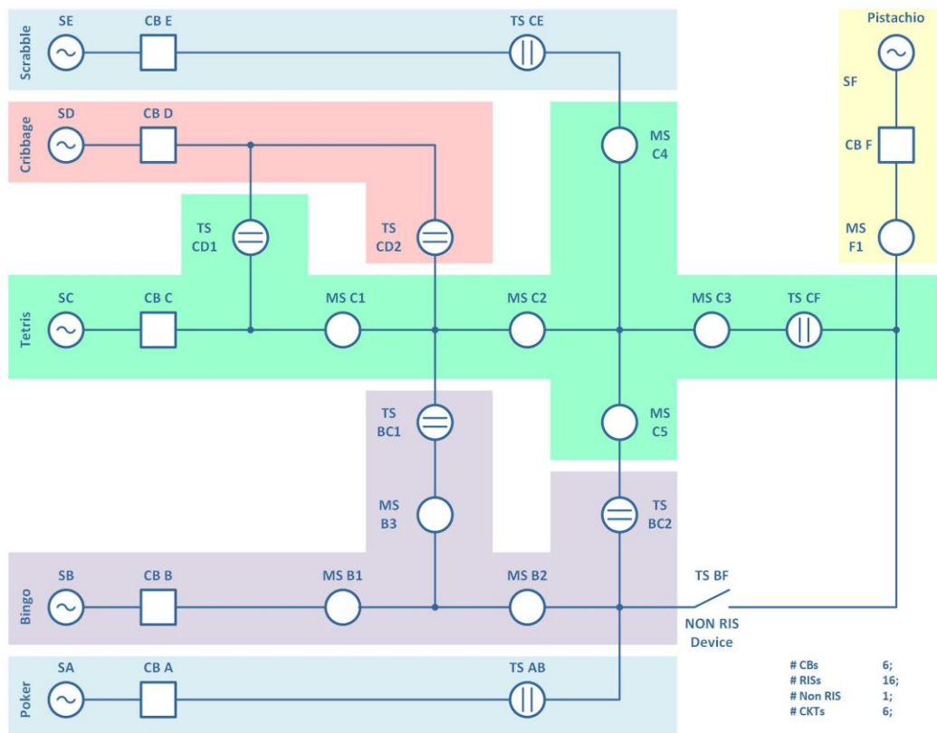
Fig. 1. RIS System Topology
