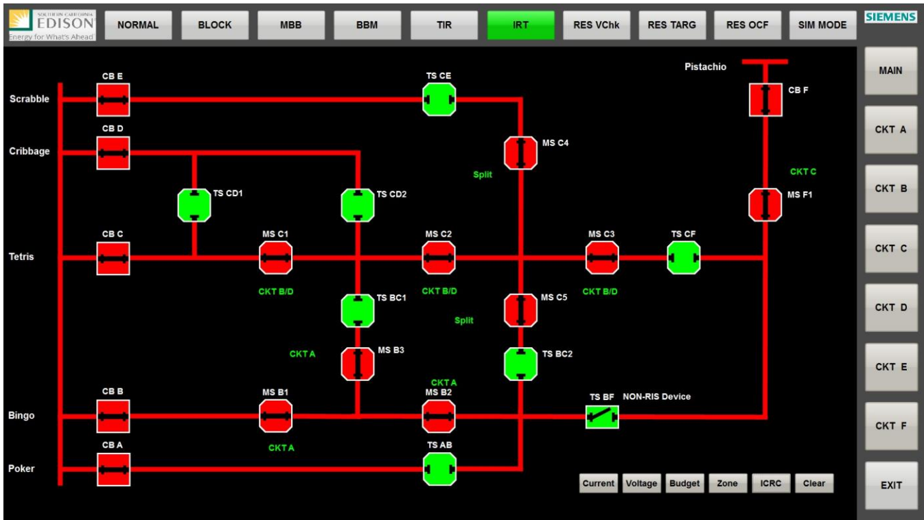
Fig. 9. Main HMI Screen
