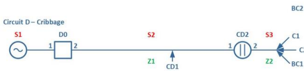
Fig. 6. RIS Circuit D
