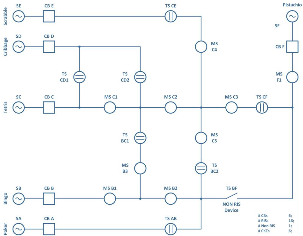
Fig. 1. RIS System Topology
