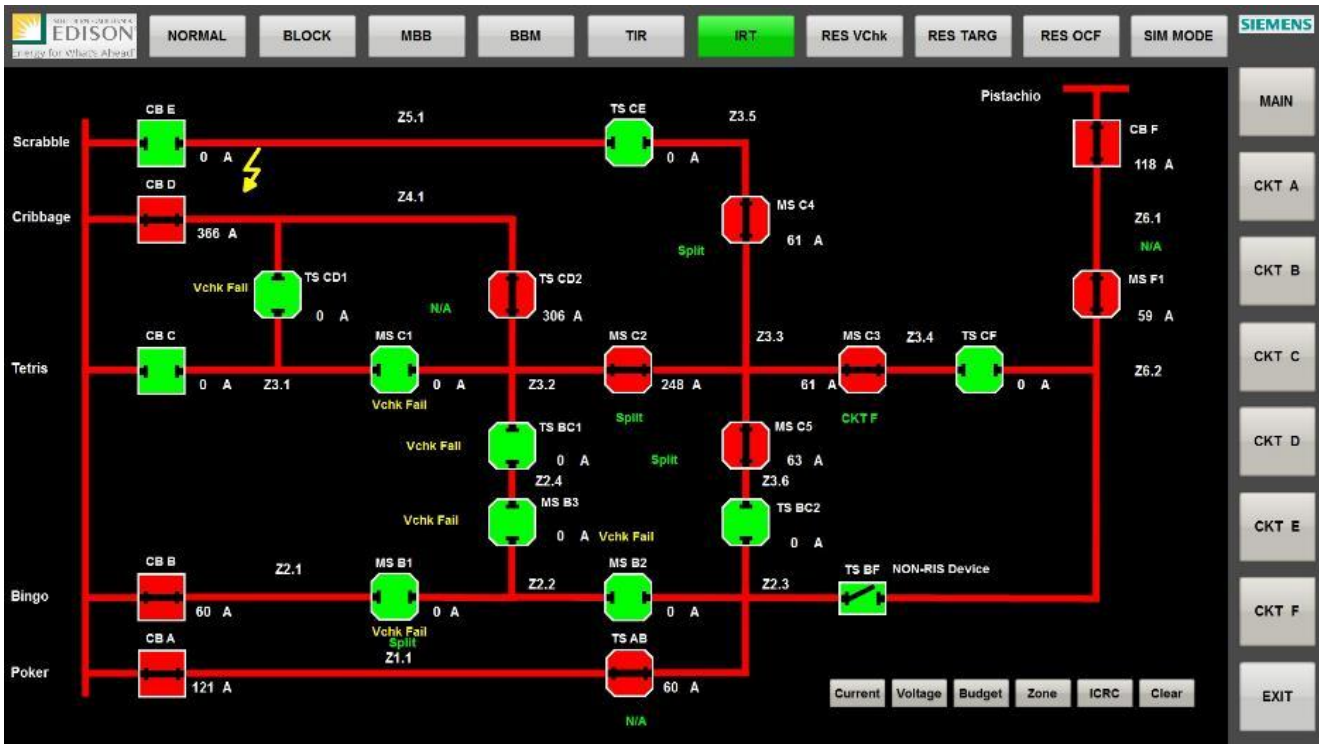
Fig. 15. System response to evolving fault in Zone 5.1
