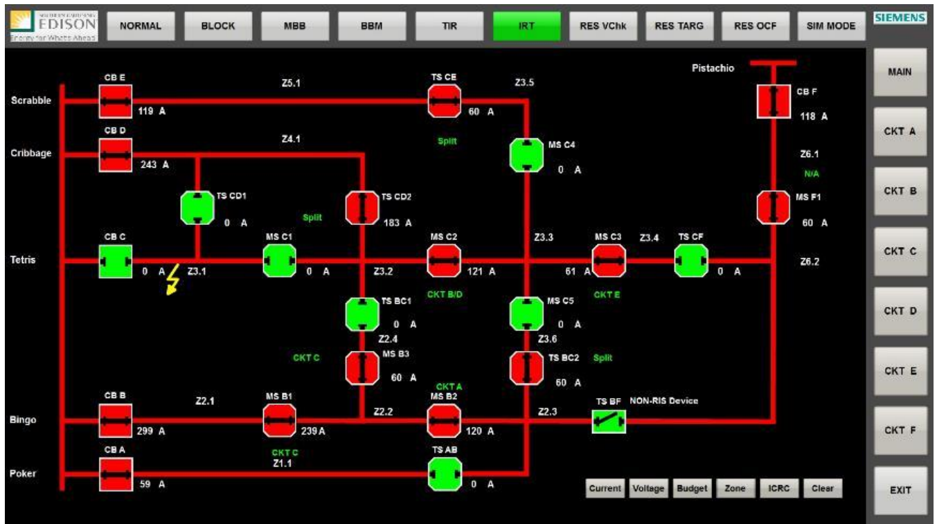
Fig.13. System response to a fault in Zone 3.1
