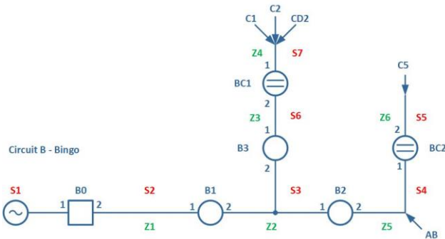
Fig. 4. RIS Circuit B
