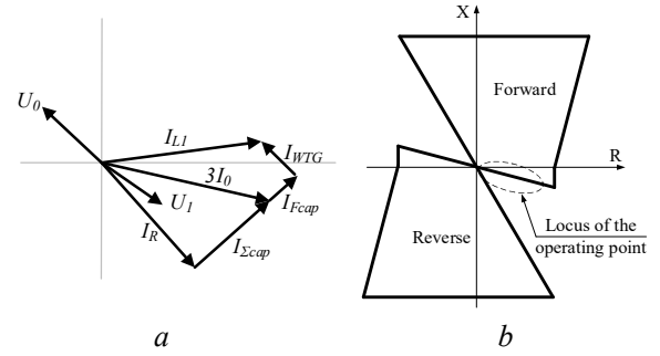
Fig. 2 Array cable exposed to an earth fault (a) phasor diagram at the distance protection location, (b) potential locus of the operating point in the 4 th quadrant
