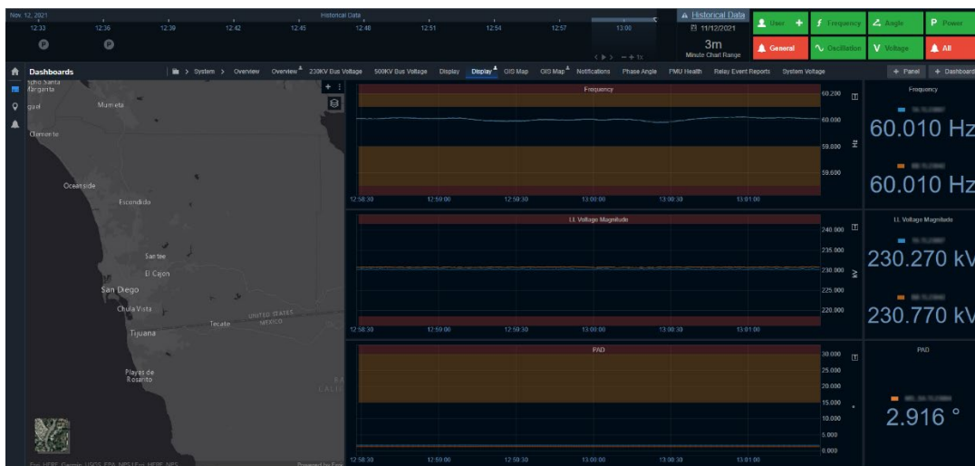
Figure 7: Typical WASA display for system operator
