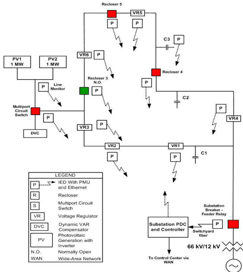
Figure 3: FCP circuit IED deployment example
