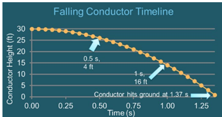
Figure 2: Distribution falling conductor protection (DFCP) operational timing
