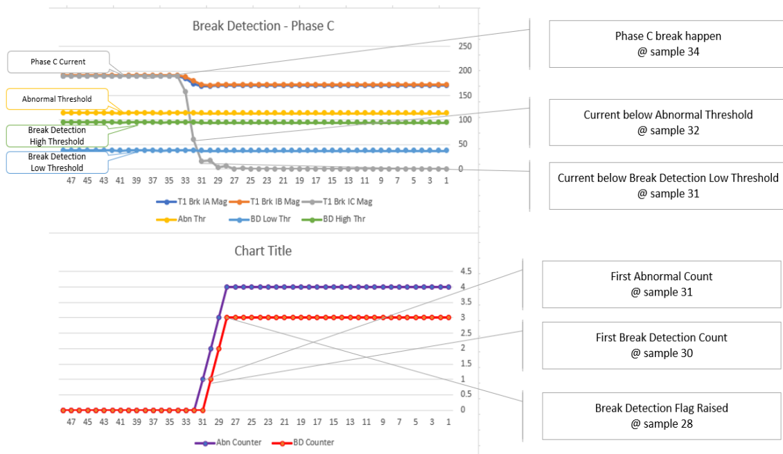
Figure 16: Example TFCP test result
