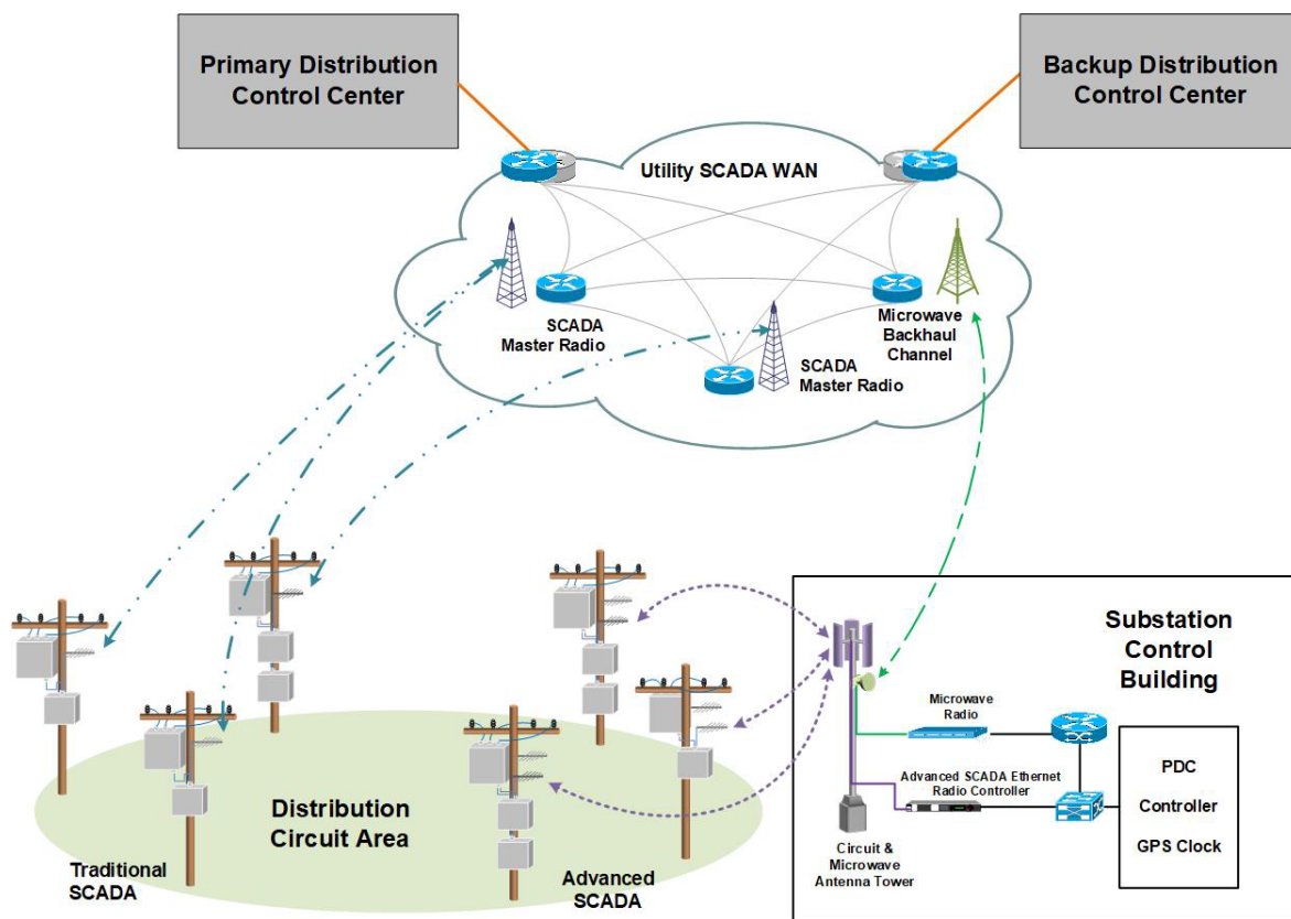
Figure 4: FCP radio communications architecture
