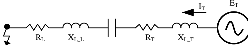
Figure 24. Simplified system
