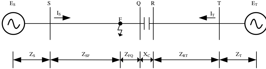
Figure 16. A system with a series capacitor bank
