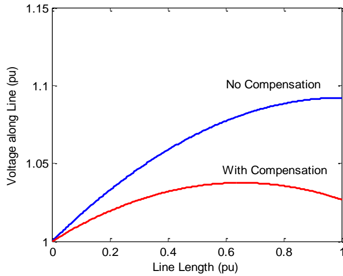
Figure 3. Voltage profile when shunt reactor compensation applied
