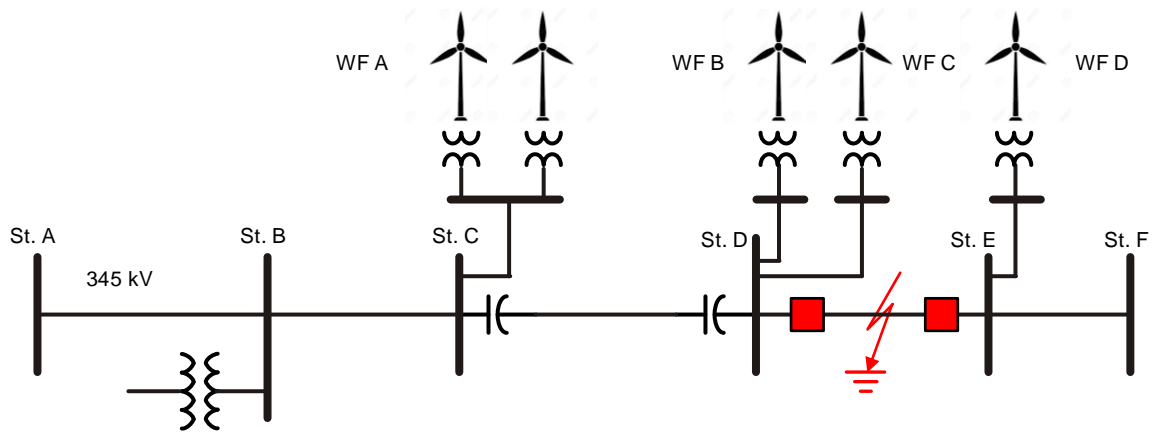
Figure 15. Case #2 single line diagram
