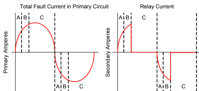
Fig. 6. Currents for an internal fault with 87Z element in service
