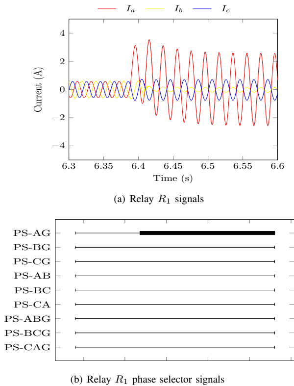
Fig. 21: Relay R_1 event recorded for a cross country fault F_1 = AG and F_2 = BG
