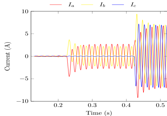
(b) Current signals
