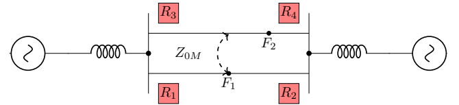
Fig. 19: Cross country fault on double circuit line
