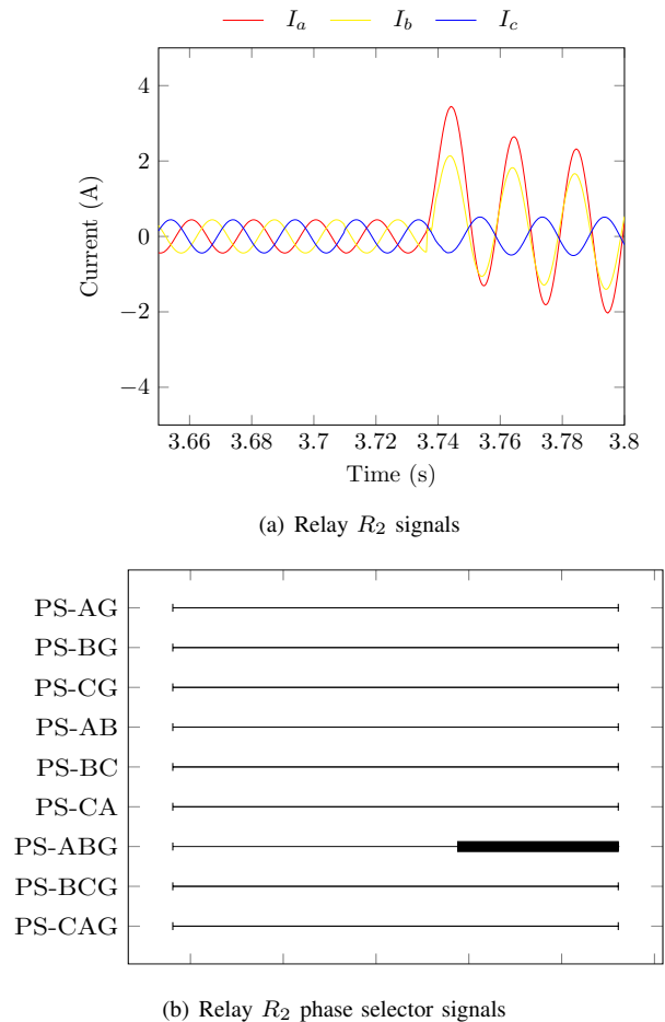
Fig. 23: Relay R_2 events- cross country fault F_1 = AG & F_2 = ABG (Fig. 19)
