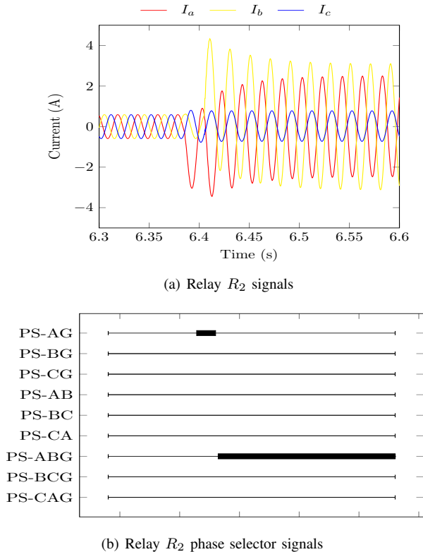
Fig. 22: Relay R_2 events- cross country fault F_1 = AG & F_2 = BG
