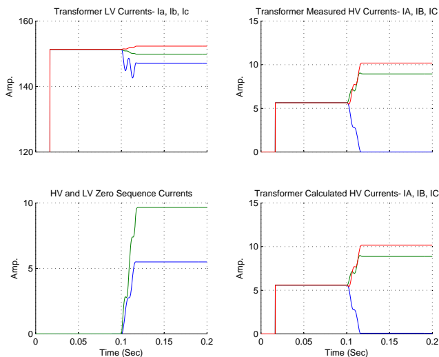
Fig. 27. Simulation Results for Measured and Calculated Primary Currents in a Three-leg core Y_g - Y_g Transformer After Loss of Phase A- Load=120KW
