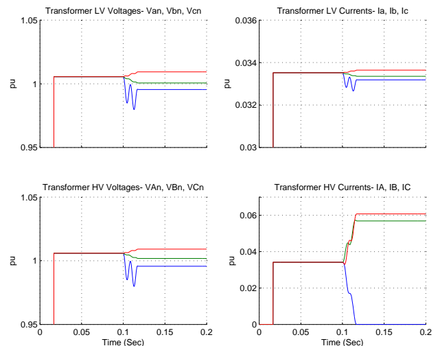
Fig. 17. Simulation Results for a Three-leg Y_g - Y_g Transformer After Loss of Phase A- Load=60KW
