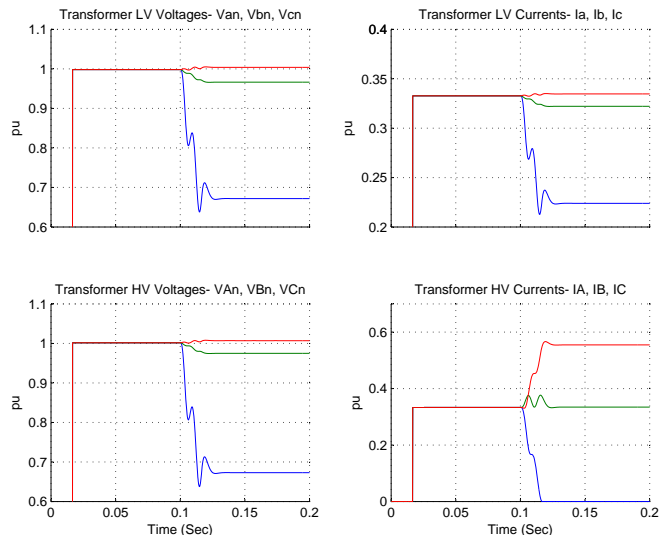
Fig. 18. Simulation Results for a Three-leg Y_g - Y_g Transformer After Loss of Phase A- Load=600KW
