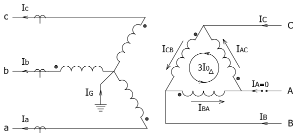
Fig. 25. Currents in a \Delta - Y_g Transformer with D11 Primary
