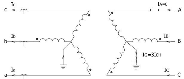
Fig. 26. Currents in a Y_g - Y_g Transformer
