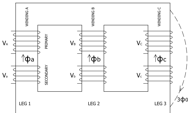
Fig. 1. Three-Leg Core Type Transformer
