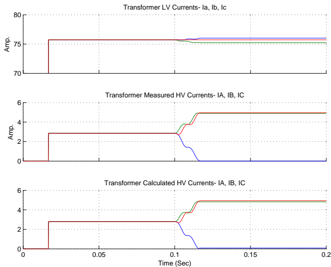
Fig. 22. Simulation Results for Measured and Calculated Primary Currents in a Y_g - \Delta Transformer After Loss of Phase A- Load=60KW
