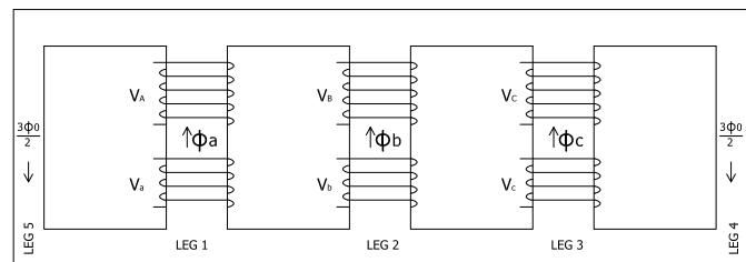
Fig. 3. Five-Leg Core Type Transformer
