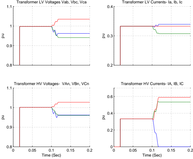
Fig. 12. Simulation Results for a Y_g - \Delta Transformer After Loss of Phase A- Load=600KW
