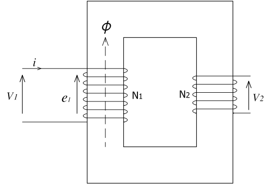
Fig. 5. Illustration of V_1 , e_1 and \phi in an Unloaded Transformer
