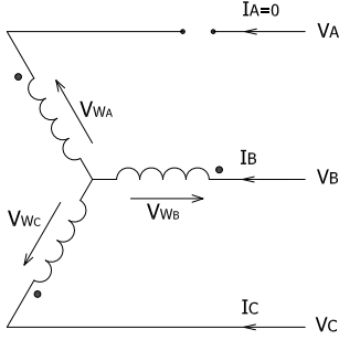
Fig. 8. Y Primary Winding with Phase A Open
