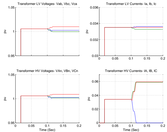
Fig. 11. Simulation Results for a Y_g - \Delta Transformer After Loss of Phase A- Load=60KW
