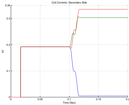
Fig. 13. Coil Currents on the Secondary Side After Loss of Phase A- Load=600KW
