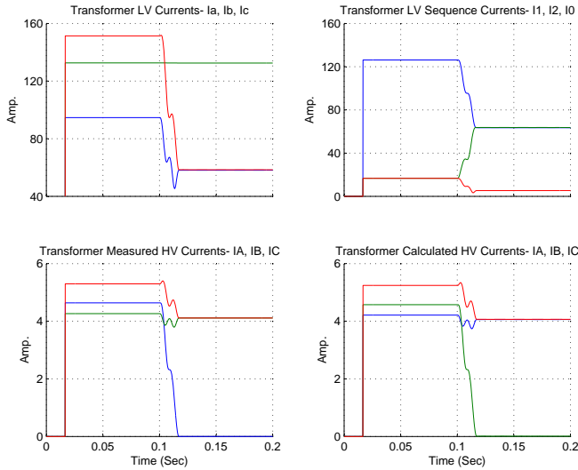
Fig. 24. Simulation Results for Measured and Calculated Primary Currents in a \Delta - Y_g Transformer After Loss of Phase A- Unbalanced Load=100KW
