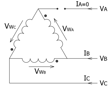
Fig. 7. \Delta Primary Winding with Phase A Open
