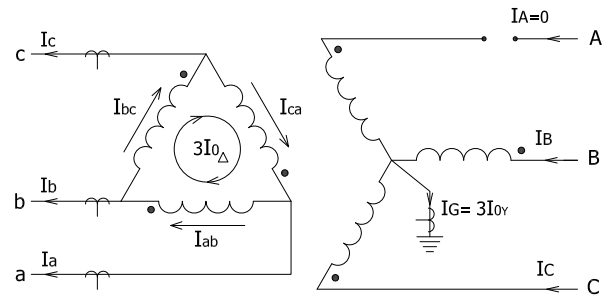
Fig. 21. Y_g - \Delta Transformer with D11 Secondary Winding
