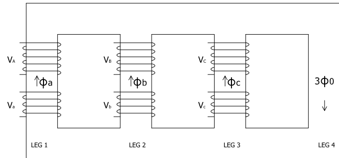
Fig. 2. Four-Leg Core Type Transformer
