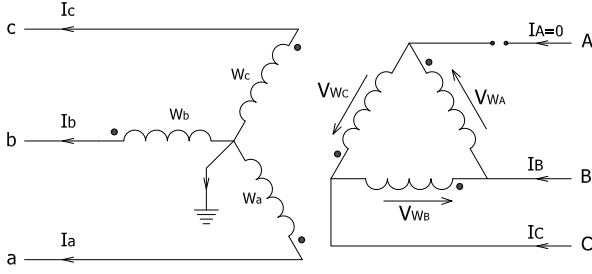
Fig. 14. \Delta - Y_g Transformer with Phase A Open on the High Side
