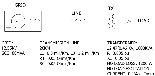
Fig. 10. Single Line Diagram of the Sample Power System
