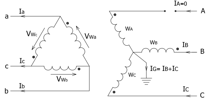
Fig. 9. Open Phase in a Y_g - \Delta Transformer
