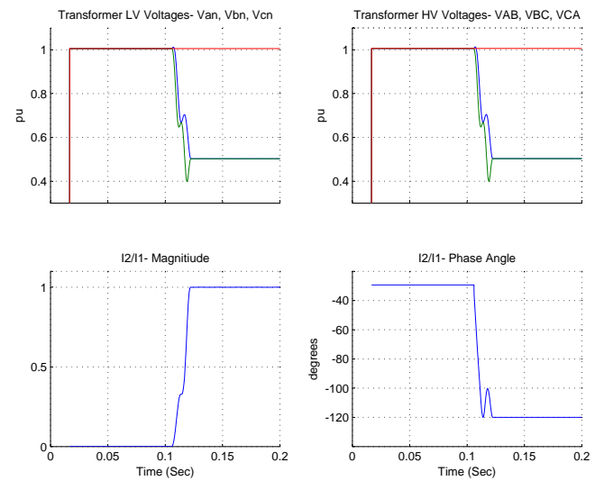
Fig. 15. Simulation Results for a \Delta - Y_g Transformer After Loss of Phase B- Load=100KW
