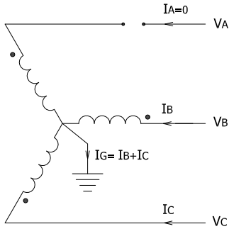
Fig. 6. Y_g Primary Winding with Phase A Open
