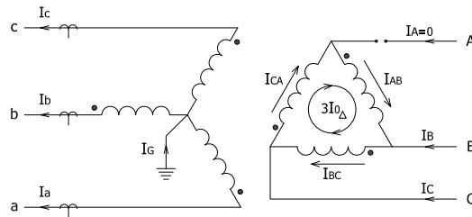
Fig. 23. Currents in a \Delta - Y_g Transformer with D1 Primary
