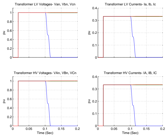
Fig. 19. Simulation Results for a Five-leg Y_g - Y_g Transformer After Loss of Phase A- Load=600KW
