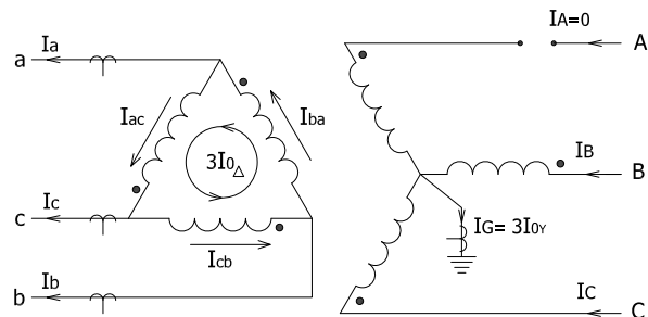
Fig. 20. Y_g - \Delta Transformer with D1 Secondary Winding
