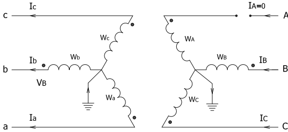
Fig. 16. Y_g - Y_g Transformer With an Open Phase
