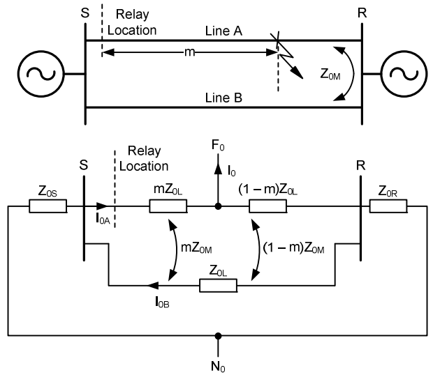
Fig. 7. System configuration and zero-sequence network for two mutually coupled lines
