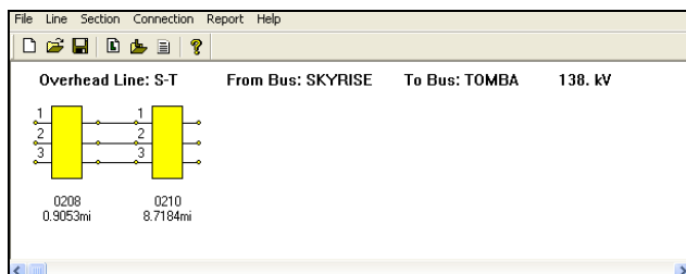
Fig. 2. ASPEN Line Constants Program screen capture showing two line sections with different tower configurations
