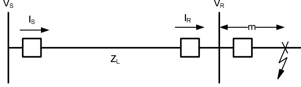
Fig. 12. Solving for line impedances for an external fault
