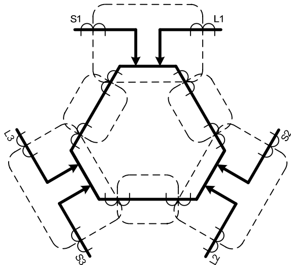
Fig. 4. Differential protection for single-core PST, 87P
