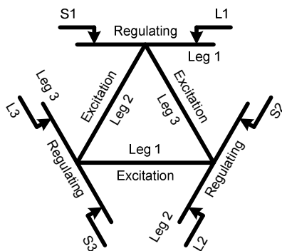
Fig. 1. Extended-delta single-core PST
