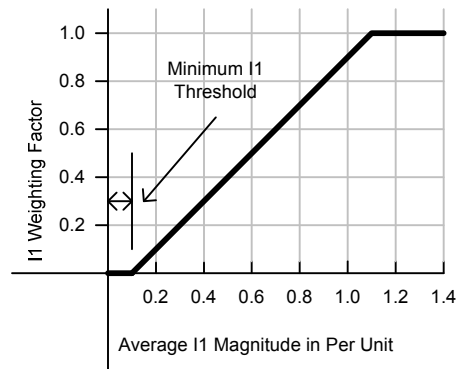
Fig. 10. I1 versus V1 angle measurement weighting factor
