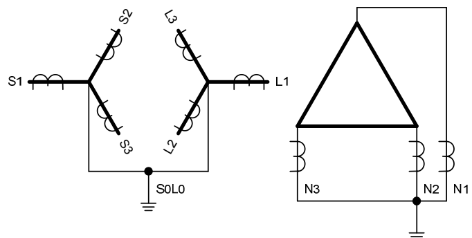
Fig. 6. Secondary differential protection for two-core PST, 87S
