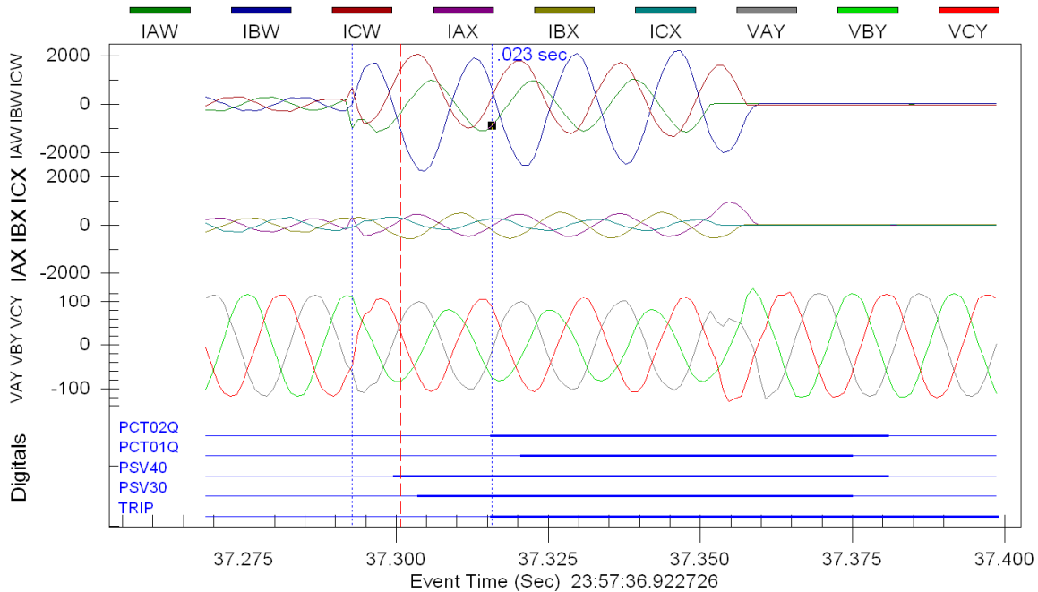
Fig. 7. Turn-to-turn fault in delta/hex PST during capacitor switching transient
