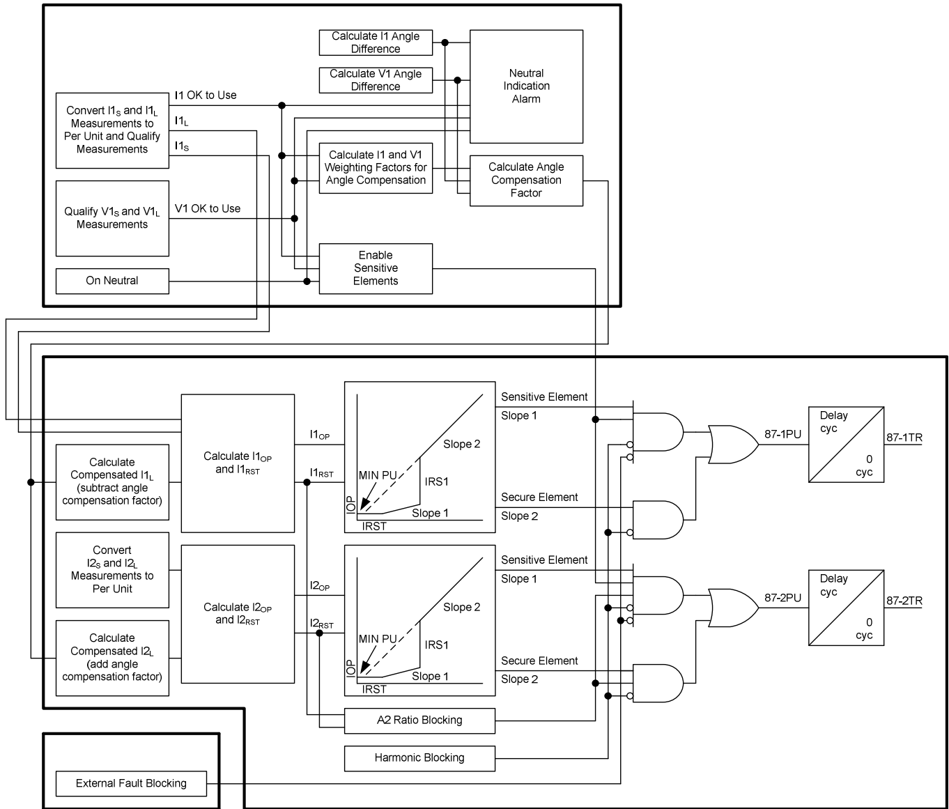
Fig. 9. Functional block diagram of PST differential protection system
