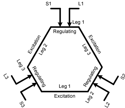
Fig. 2. Delta/hex single-core PST
