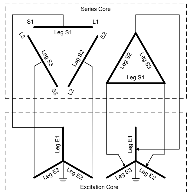
Fig. 3. Conventional two-core PST
