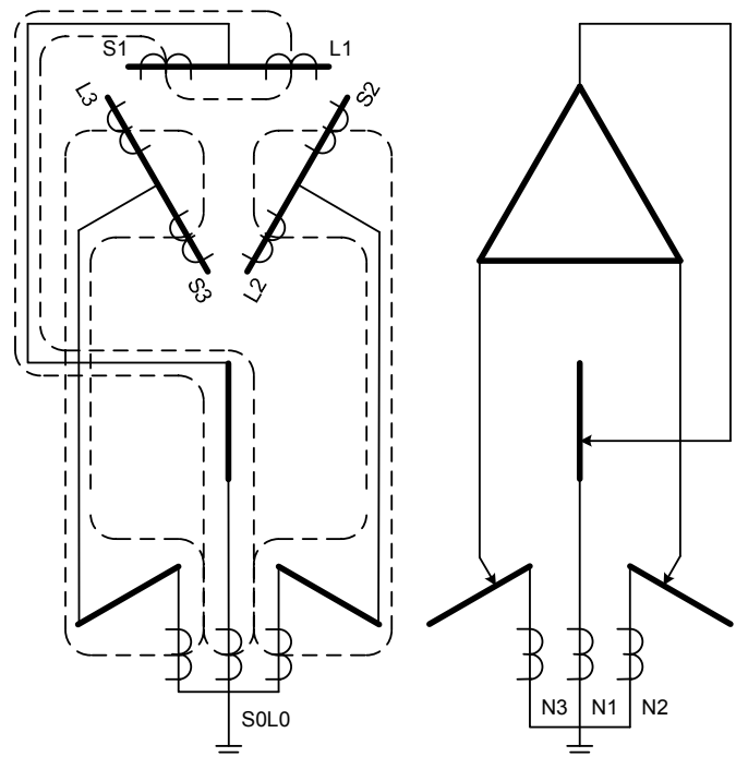
Fig. 5. Primary differential protection for two-core PST, 87P
