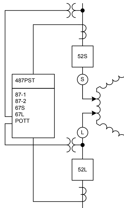
Fig. 8. Single-line diagram of PST protection system
