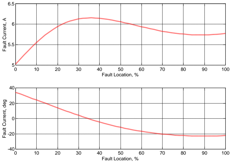
Figure 9. Fault current: magnitude (top) and phase angle (bottom).
