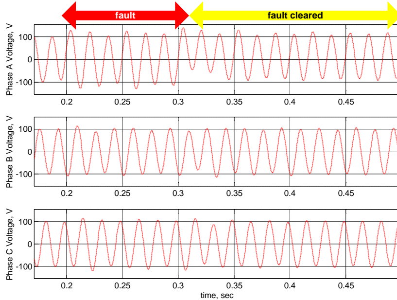
Figure 22. Sample fault on a series-compensated line: line-side VT voltages.
