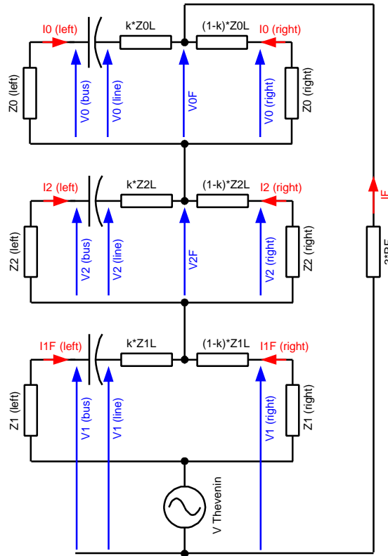
Figure 8. Sequence networks and symmetrical components for low-current SLG faults.
