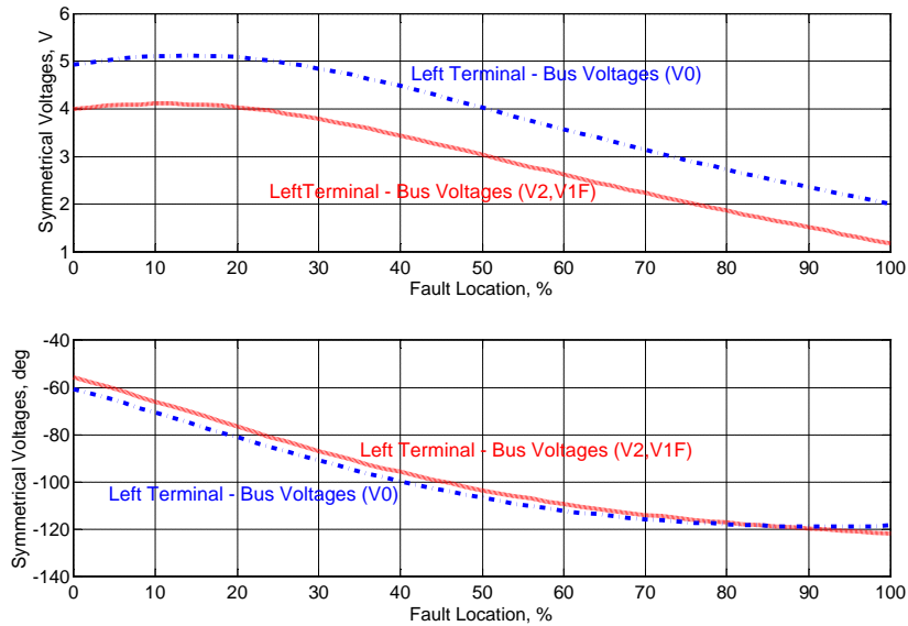
Figure 17. Symmetrical voltages – left terminal, bus side VTs: magnitude (top) and phase angle (bottom).
