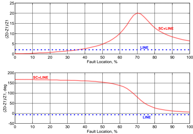
Figure 5. Zero-sequence compensating factor for a relay looking through SCs (bus potential source) at a low-current SLG fault as a function of fault location.
