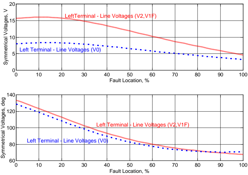
Figure 16. Symmetrical voltages – left terminal, line side VTs: magnitude (top) and phase angle (bottom).
