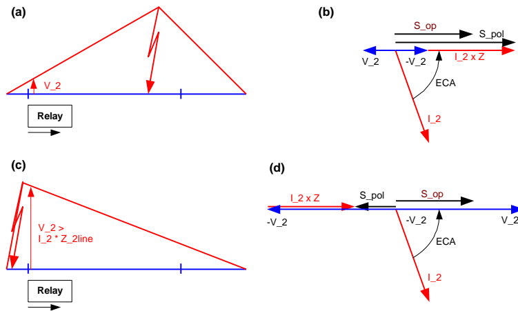
Figure 26. Negative-sequence currents and voltages for a forward ((a) and (b)) and reverse ((c) and (d)) faults.
