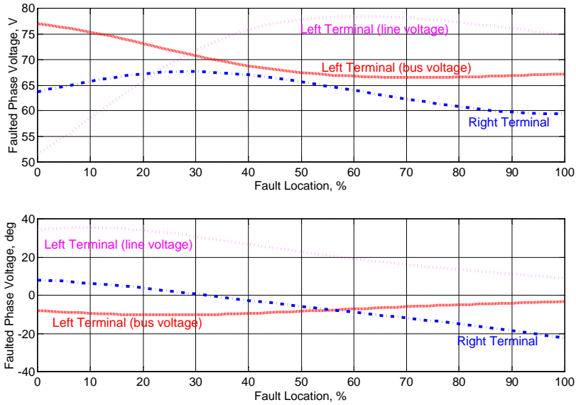
Figure 11. Faulted phase voltages: magnitude (top) and phase angle (bottom).
