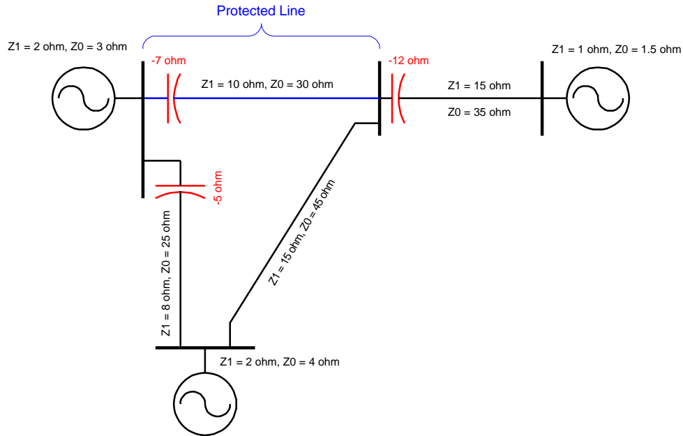
Figure 6. Sample system with series-compensated lines (secondary ohms).
