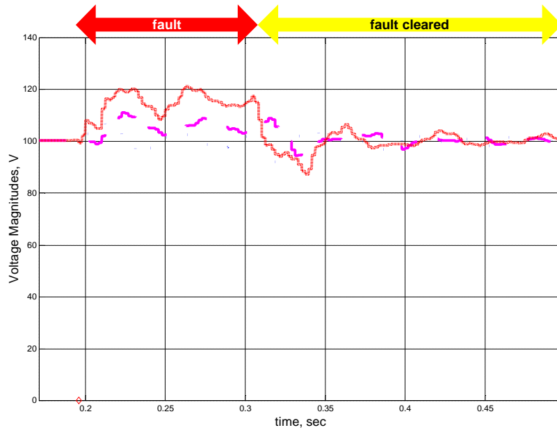
Figure 24. Sample fault on a series-compensated line: voltage magnitudes.
