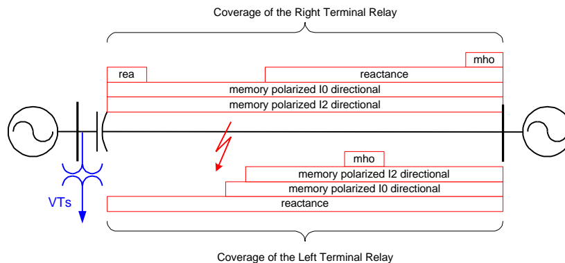
Figure 20. Coverage of various comparators while using the bus-side VTs.
