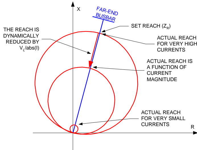
Figure 27. Current-dependent adaptive reach.
