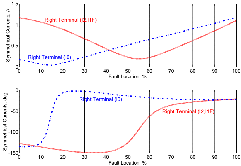
Figure 14. Symmetrical currents at the left terminal: magnitude (top) and phase angle (bottom).
