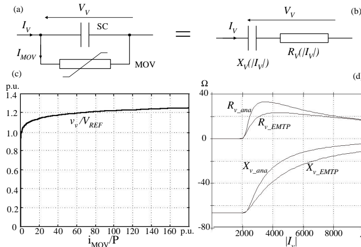
Figure 2. Series capacitors with MOVs (a); equivalent fundamental frequency impedance (b); sample MOV characteristic (c); sample current-dependent parameters of the equivalent impedance.
