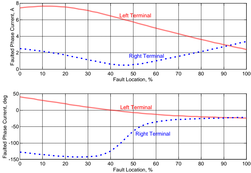
Figure 10. Faulted phase currents: magnitude (top) and phase angle (bottom).
