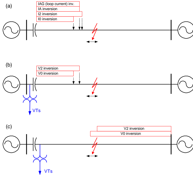
Figure 19. Fault locations causing current and voltage inversions at the left terminal relay: currents (a), voltages while using the bus-side VTs (b), and voltages while using the line-side VTs (c).
