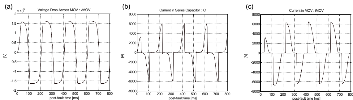
Figure 1. Voltage drop across a series capacitor with a conducting MOV (a); capacitor (b) and MOV (c) currents, respectively.
