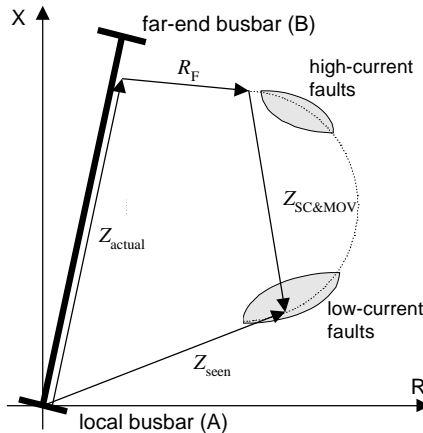
Figure 3. Distance element overreaching due to series compensation.
