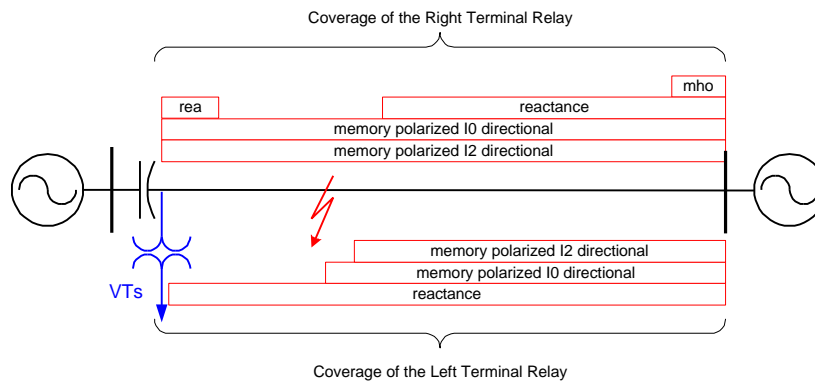
Figure 21. Coverage of various comparators while using the line-side VTs.
