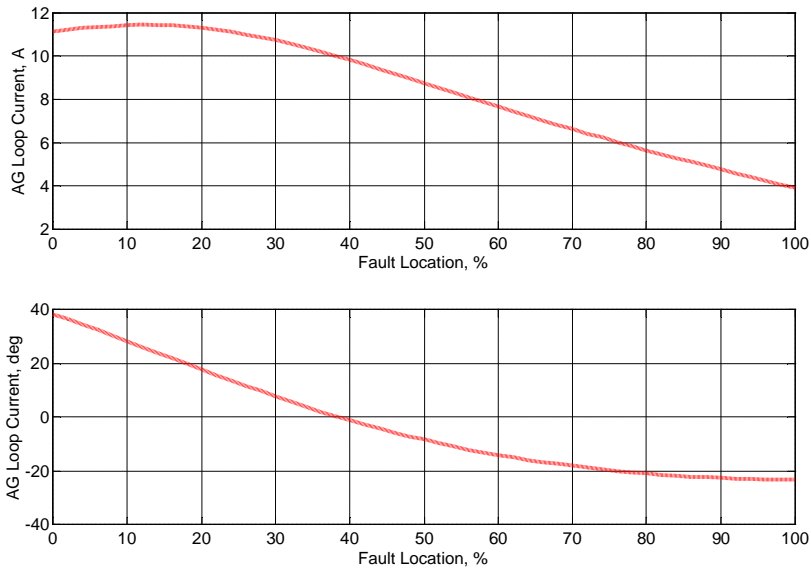
Figure 13. Fault loop current at the left terminal: magnitude (top) and phase angle (bottom).
