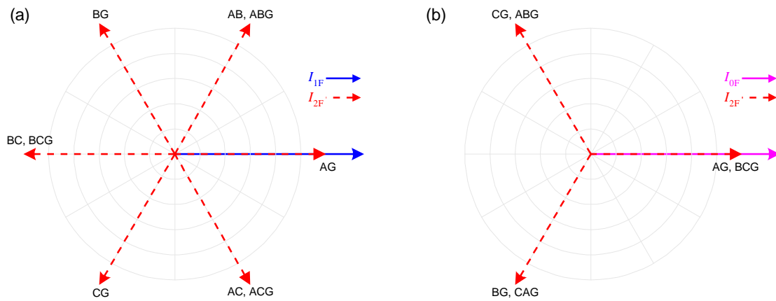
Figure 29. Negative-sequence vs. positive-sequence fault signature (a) and negative-sequence vs. zero-sequence fault signature (b).
