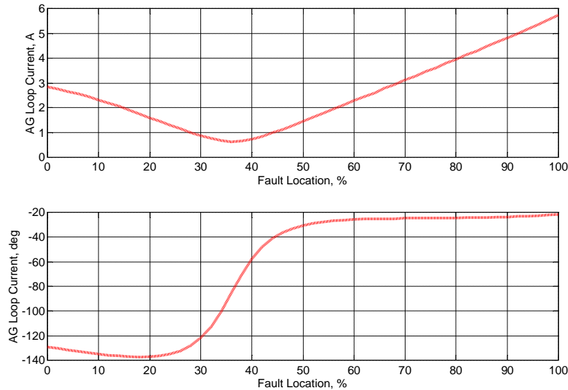
Figure 15. Fault loop current at the left terminal: magnitude (top) and phase angle (bottom).
