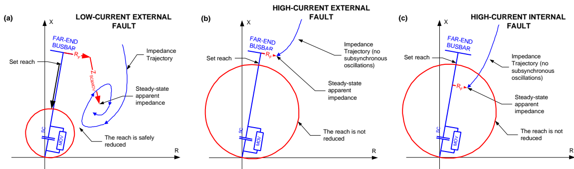
Figure 28. Illustration of the current-dependent adaptive reach.
