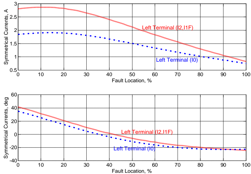
Figure 12. Symmetrical currents at the left terminal: magnitude (top) and phase angle (bottom).
