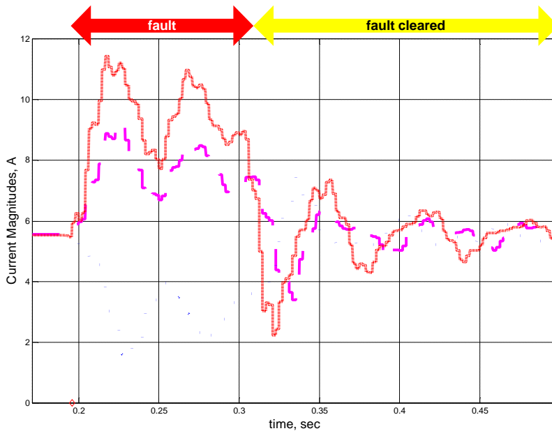
Figure 25. Sample fault on a series-compensated line: current magnitudes.
