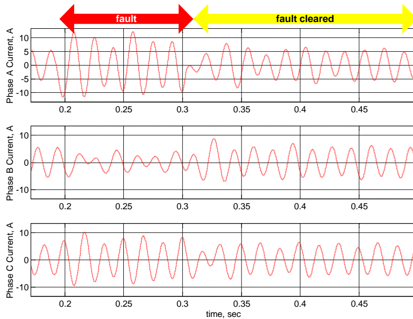
Figure 23. Sample fault on a series-compensated line: currents.
