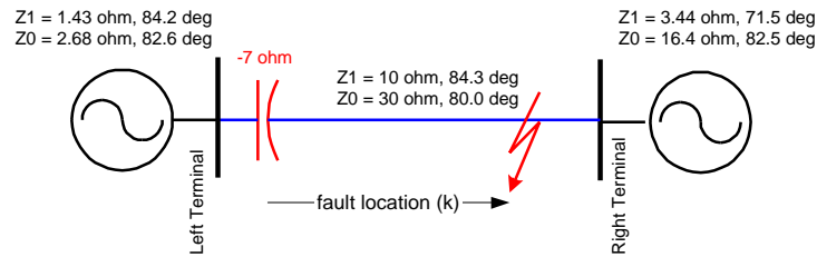
Figure 7. Equivalent of the sample system for internal faults.
