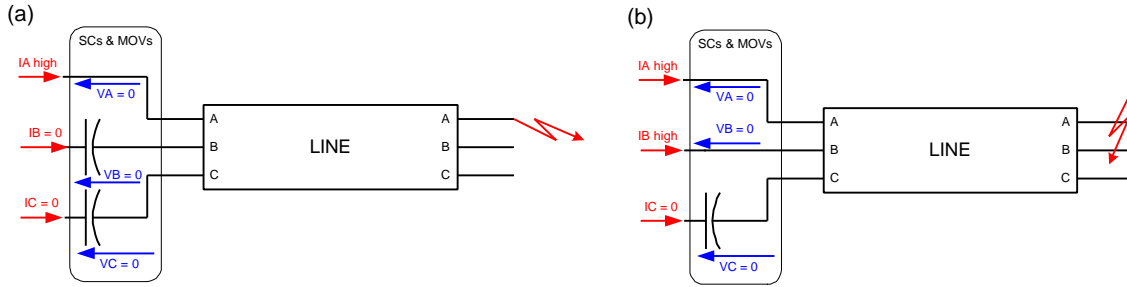
Figure 4. Voltage drops across the SC banks during high-current faults: SLG faults (a) and LL/LLG faults (b).
