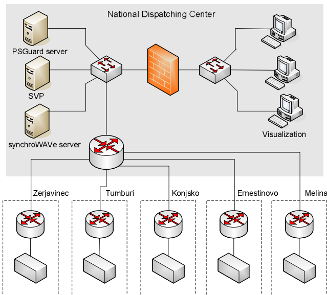
Fig. 5. WAM system architecture
