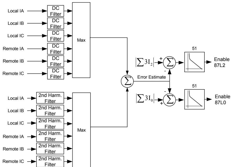
Figure 24 CT Saturation Security Supervision for 87L2 and 87LG Elements
