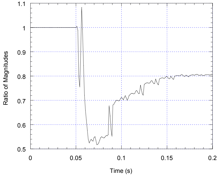
Figure 19 Ratio of Magnitudes of I_{A\_sat} Over I_A
