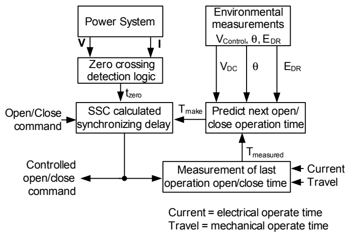
Fig. 3. Block diagram of controlled switching
