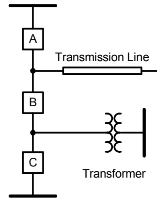
Fig. 15. Breaker-and-a-half bus configuration with a transformer and a line
