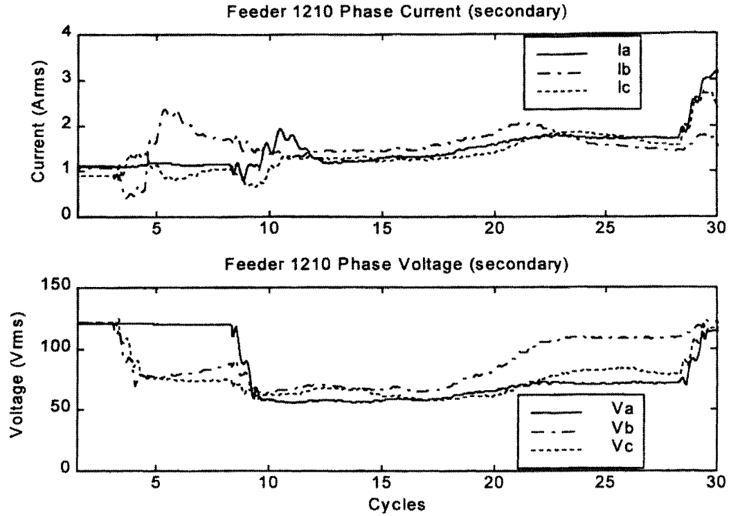
Figure 5: Phase Voltages and Currents Measured by the Feeder 1210 Relay
