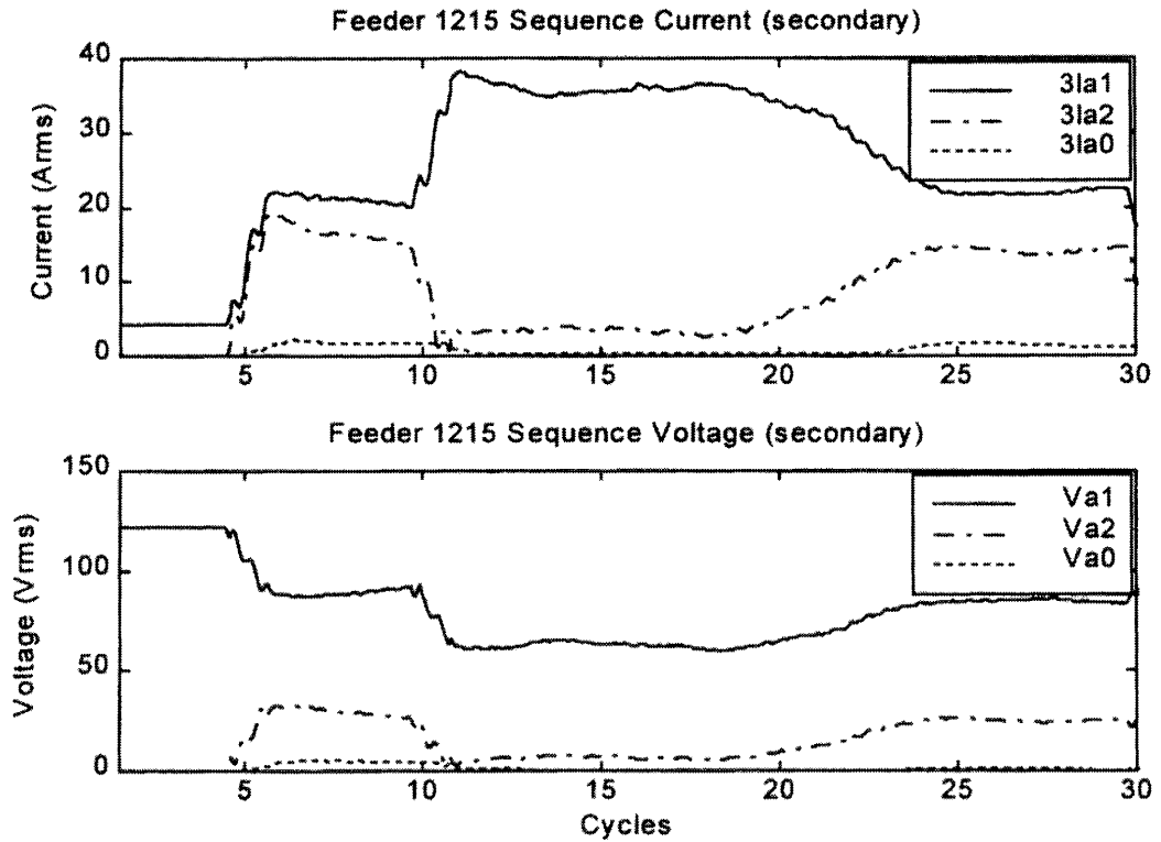
Figure 8: Sequence Voltages and Currents Measured by the Feeder 1215 Relay
