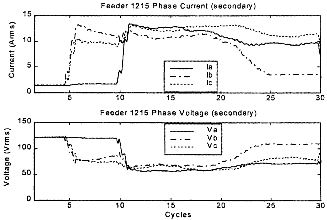
Figure 6: Phase Voltages and Currents Measured by the Feeder 1215 Relay
