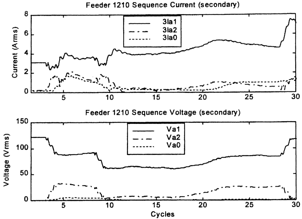
Figure 7: Sequence Voltages and Currents Measured by the Feeder 1210 Relay
