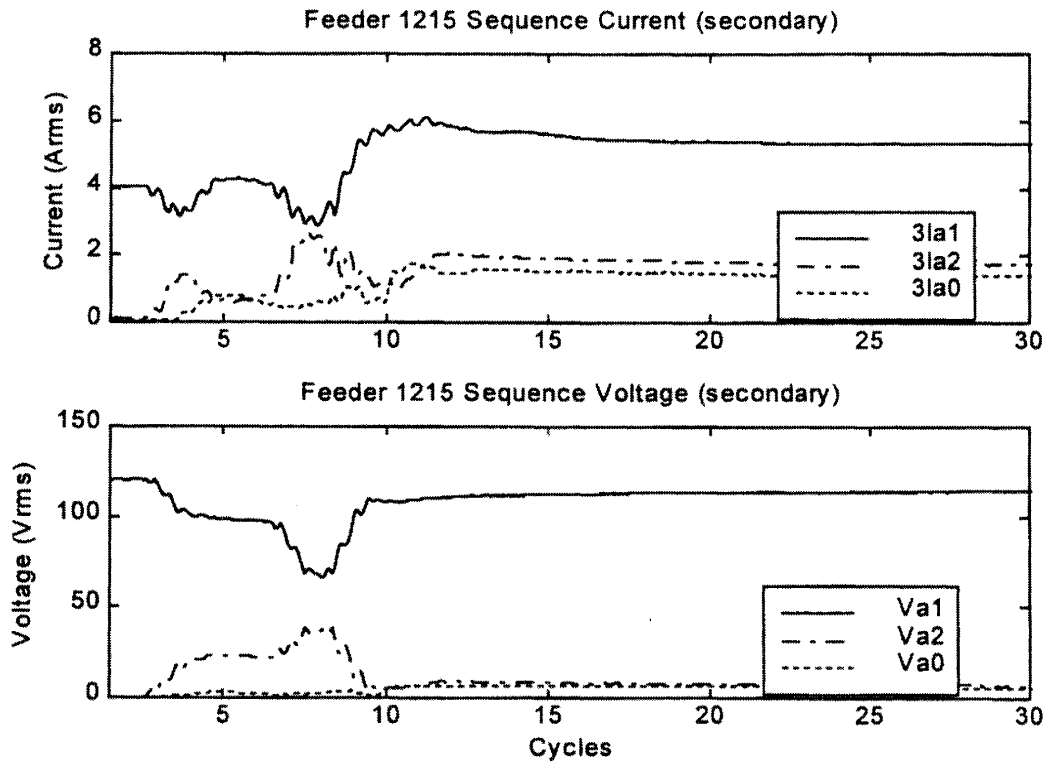
Figure 12: Sequence Voltages and Currents Measured by the Feeder 1215 Relay
