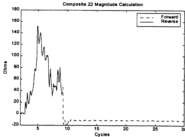
Figure 24: Composite 32Q Directional Element Calculation Results for Feeder 1215 Relay During and After the NPC 69 kV Ground Fault
