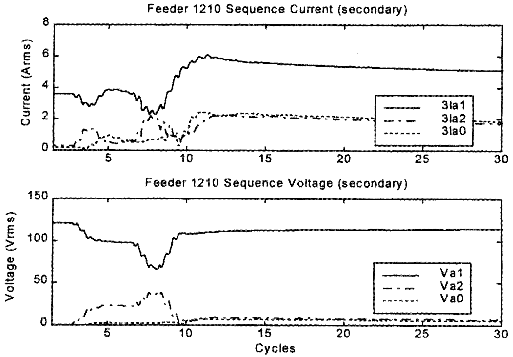
Figure 14: Sequence Voltages and Currents Measured by the Feeder 1210 Relay
