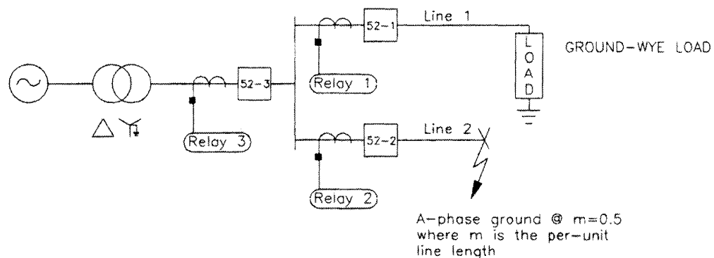
Figure 1: Single-Line Diagram for an Adjacent Feeder Fault on a Radial System
