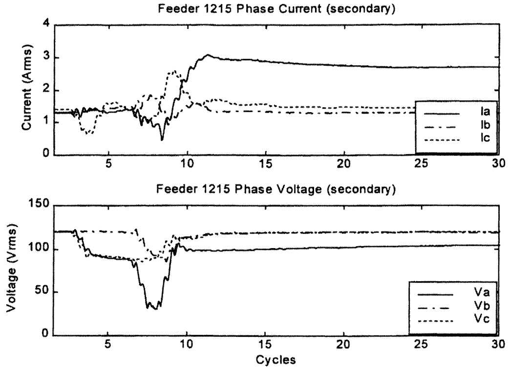
Figure 11: Phase Voltages and Currents Measured by the Feeder 1215 Relay
