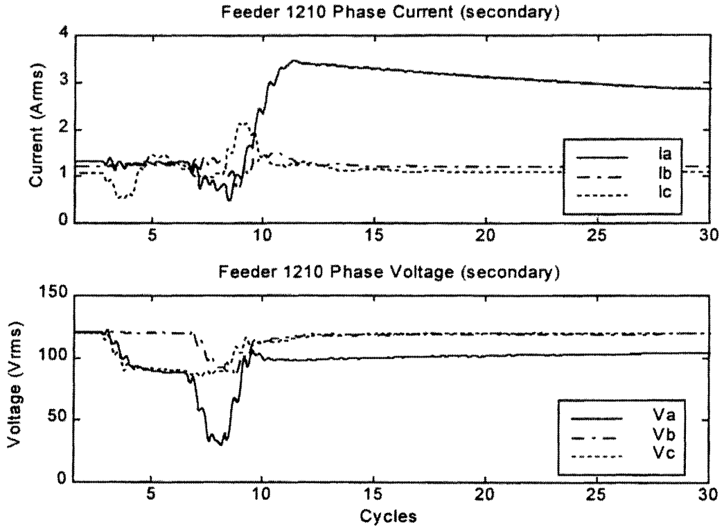
Figure 13: Phase Voltages and Currents Measured by the Feeder 1210 Relay
