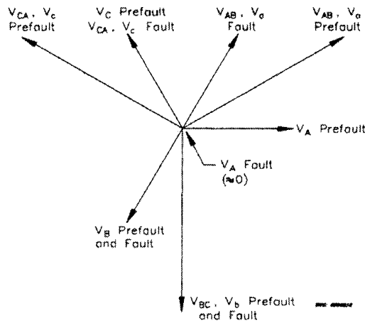
Figure 15: Feeder Relay Voltages Measured for an A-Phase-Ground Fault on the High Voltage Side of a Delta-Wye-Grounded Transformer
