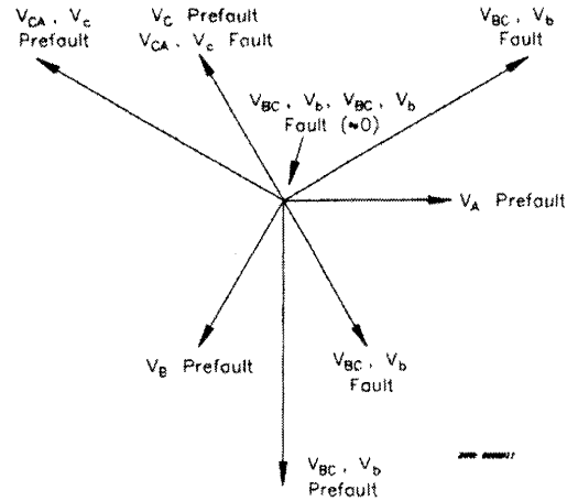
Figure 16: Feeder Relay Voltages Measured for an AB-Phase-Ground Fault on the High Voltage Side of a Delta-Wye-Grounded Transformer
