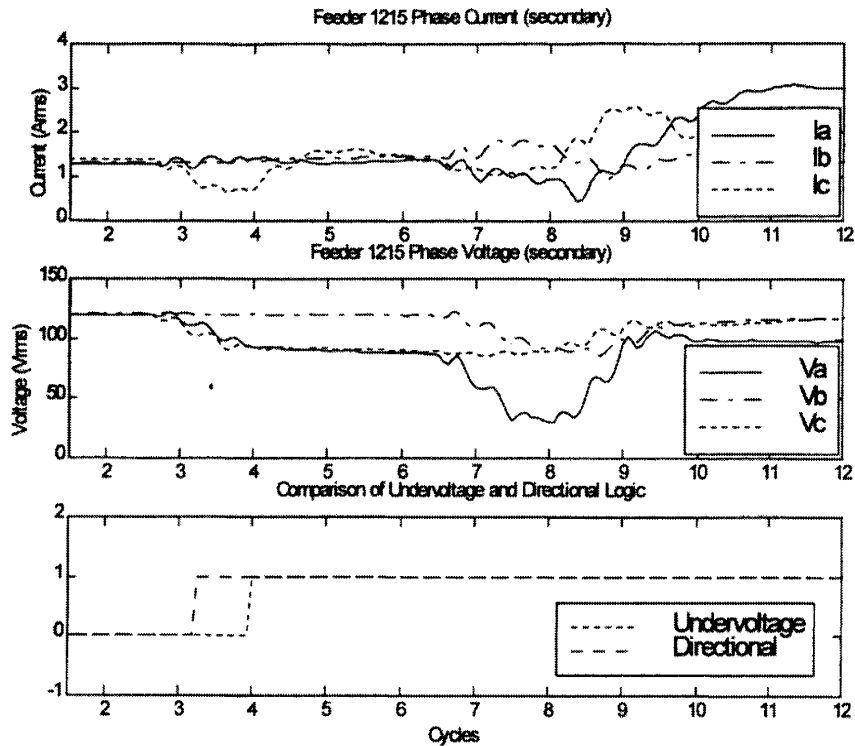
Figure 25: Performance Comparison of the Two New Sympathetic Trip Logics
