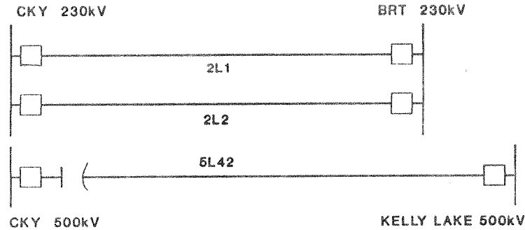
Figure 8. CKY, BRT, and Kelly Lake System Diagram
