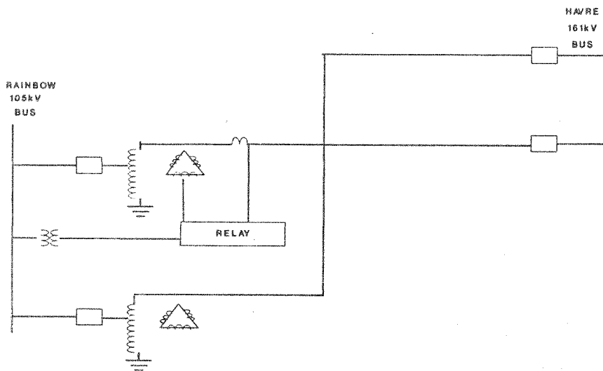
Figure 17. Rainbow-Havre Single Line Diagram
