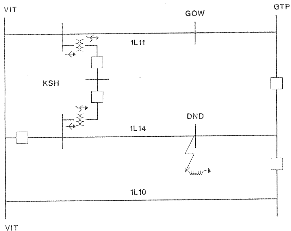
Figure 21. VIT and GTP System Single Line Diagram
