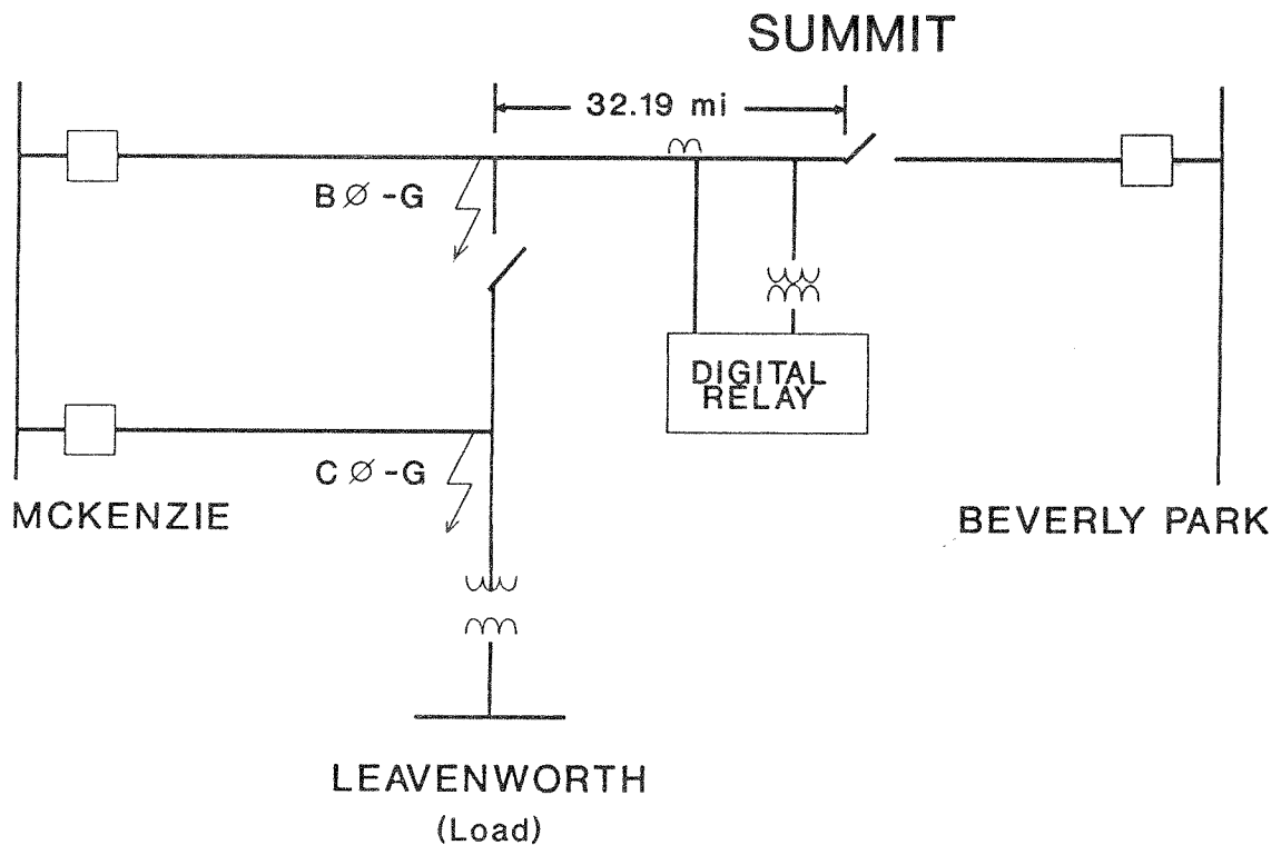
Figure 24. McKenzie-Summit Single Line Diagram
