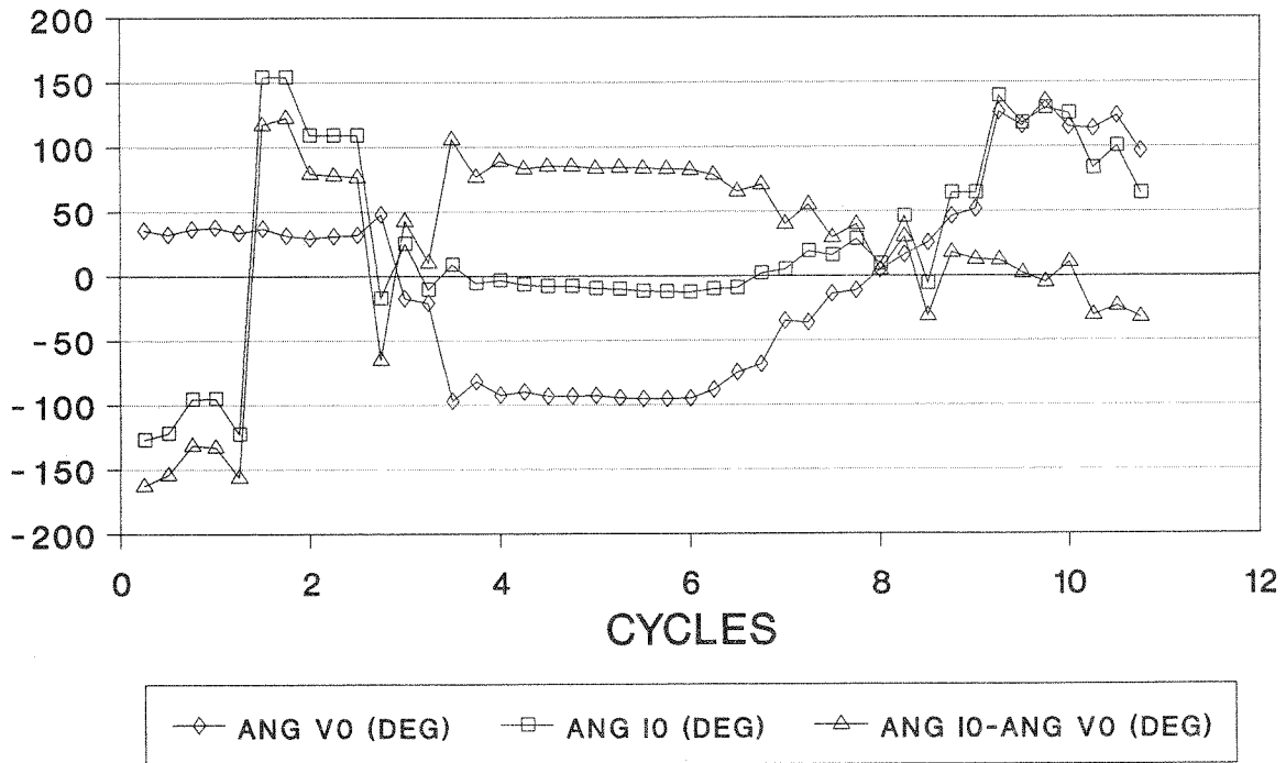
Figure 10. I_0 vs V_0 for CKY 230kV Terminal
