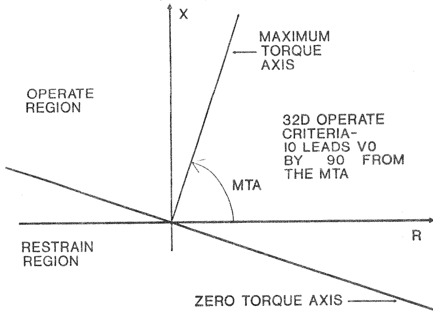
Figure 9. Operate and Restrain Regions of Zero Sequence Directional Element
