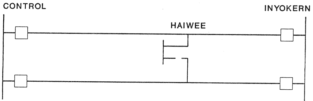
Figure 18. CONTROL - INYOKERN 115kV Transmission System Single Line
