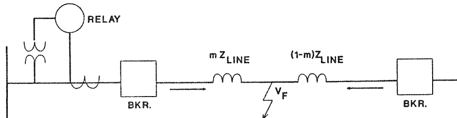
Figure A1. A\phi -Ground Fault
