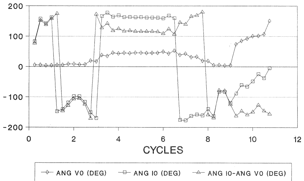
Figure 11. I_0 vs V_0 for BRT 230kV Terminal
