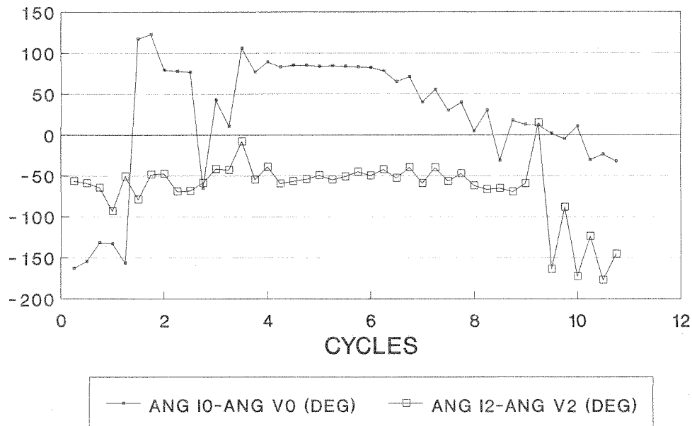
Figure 12. I_2 vs V_2 Comparison with I_0 vs V_0 at the CKY Terminal
