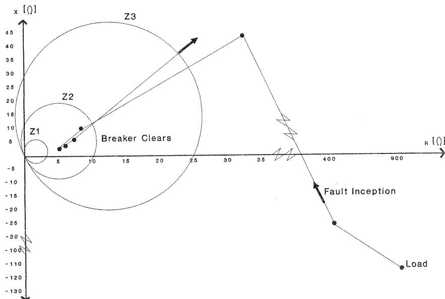
Figure 6. Lea County Electric Event Report R-X Diagram
