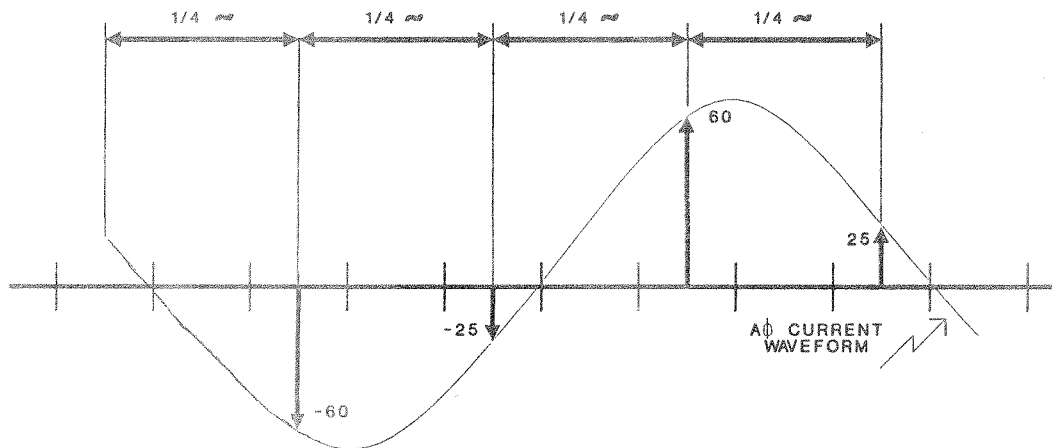
Figure 3. First Cycle of A \phi Current Samples, Incorrect Wiring Event Report
