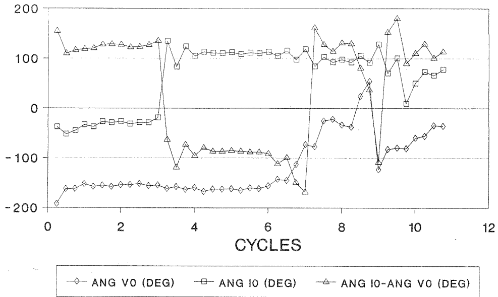
Figure 22. VIT V_0 vs I_0 Graph Showing Forward to Reverse Fault
