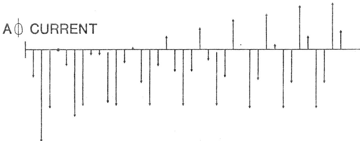
Figure 15. A \phi Current Waveform from Event 6
