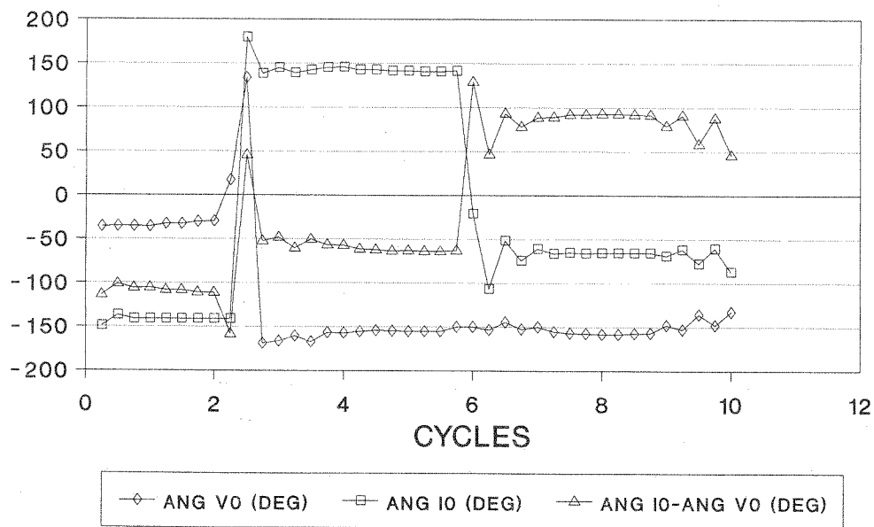
Figure 23. GOW V_0 vs I_0 Graph Showing Reverse to Forward Fault
