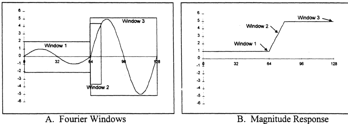
Figure 4 - Variable Width Fourier Window
