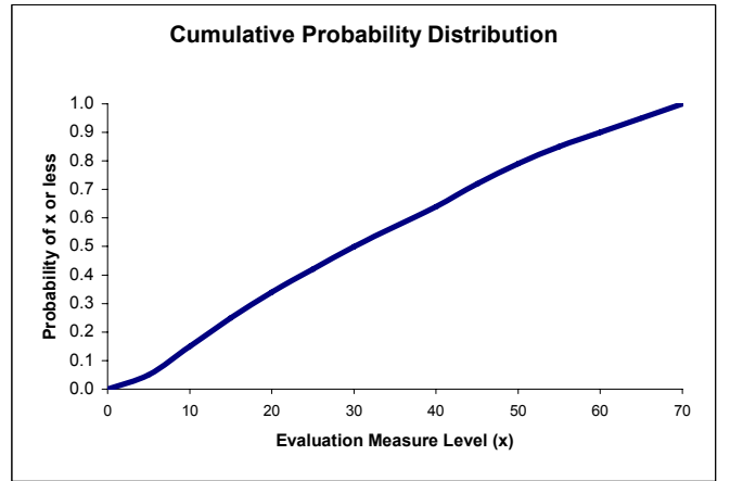
Fig. 4. Cumulative probability distribution function
