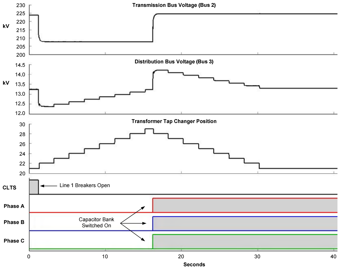
Fig. 16. RTDS Event Capture Showing Bus 2 RMS Voltage, Bus 3 RMS Voltage, Transformer Tap Changer Position, Line 1 Breaker Status, and the Capacitor Bank Breaker Status Without RECIPE Technology
