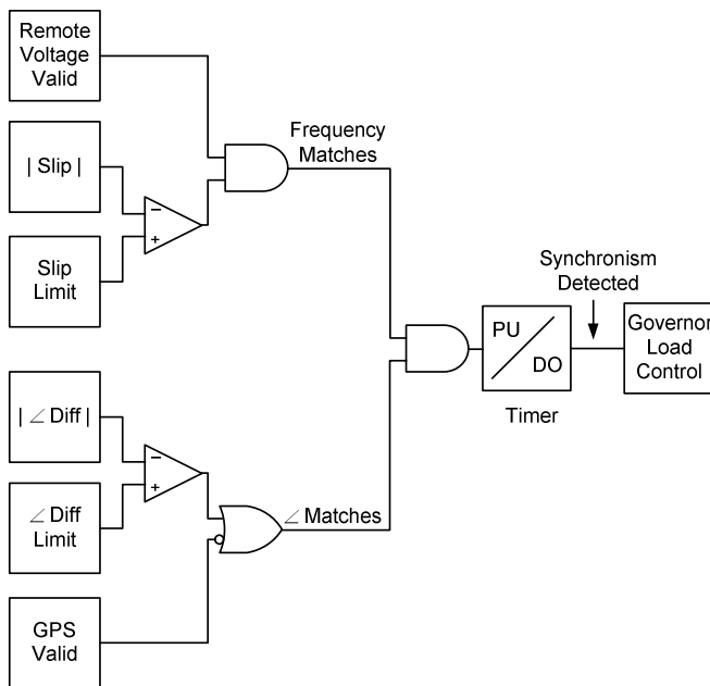
Fig. 8. Synchronism Detection Logic
