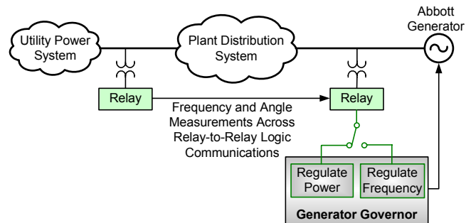
Fig. 6. Frequency and Angle Measurements Across Relay-to-Relay Logic Communications Link
