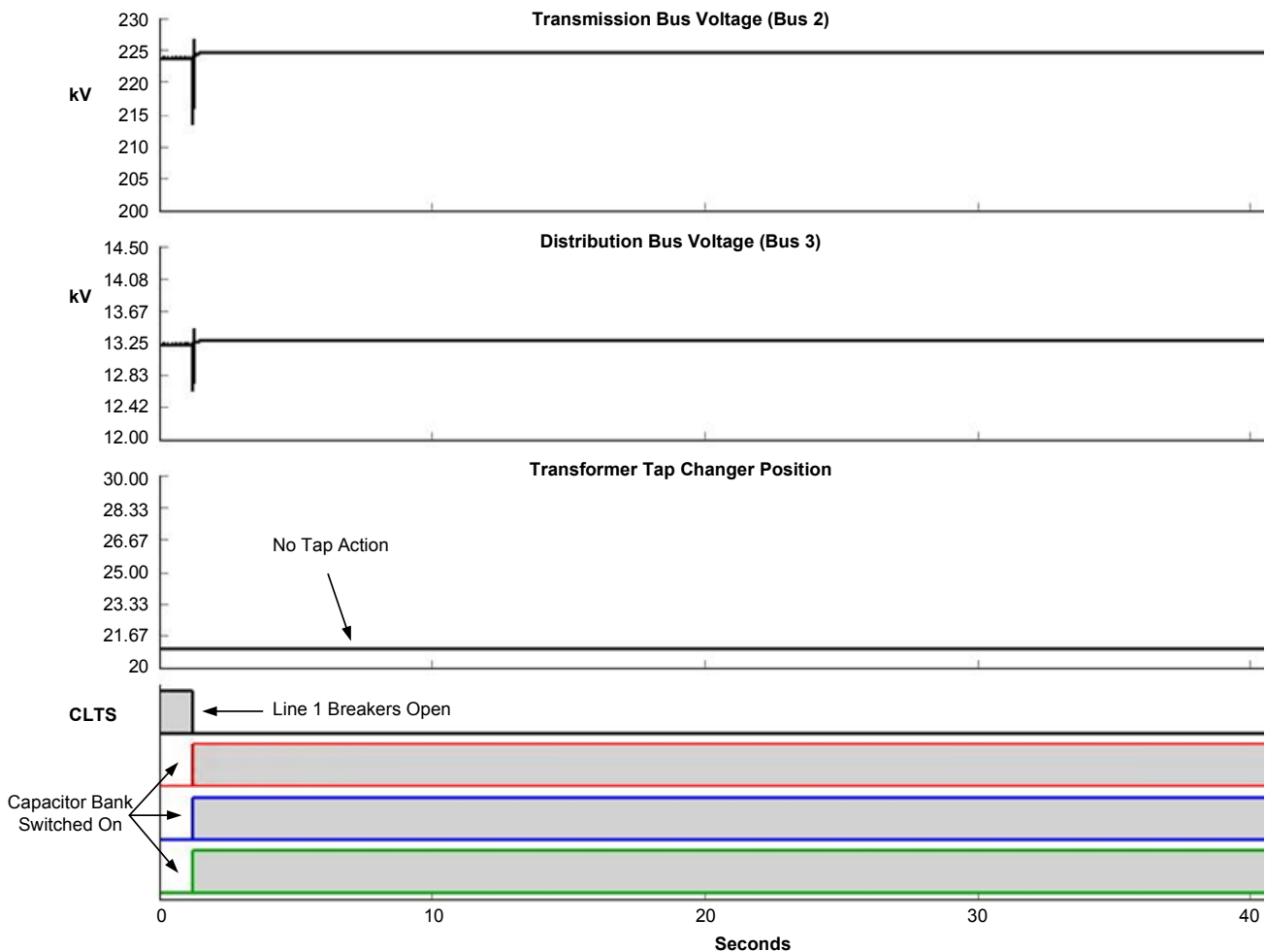
Fig. 17. RTDS Event Capture Showing Bus 2 RMS Voltage, Bus 3 RMS Voltage, Transformer Tap Changer Position, Line 1 Breaker Status, and the Capacitor Bank Breaker Status With RECIPE Technology
