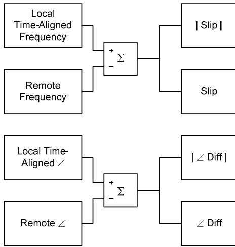
Fig. 7. Slip Frequency and Angle Differences Processed by Relays
