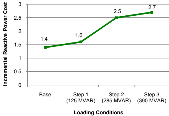
Fig. 4. QV IRPC Behavior for Different Loading Conditions [4]
