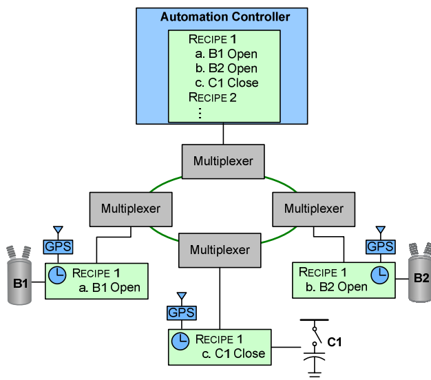
Fig. 14. RECIPE Control System
