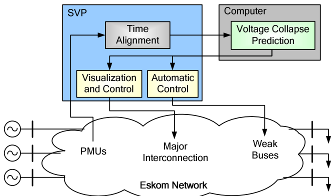
Fig. 5. Eskom's Real-Time Voltage Stability Detection and Mitigation System
