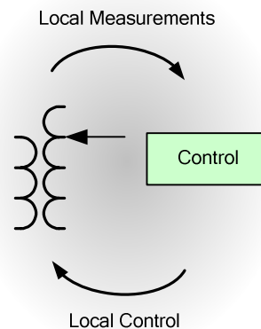
Fig. 1. Local Power Control System
