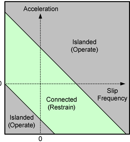
Fig. 10. Operate and Restrain Regions of the Island-Detection Characteristic
