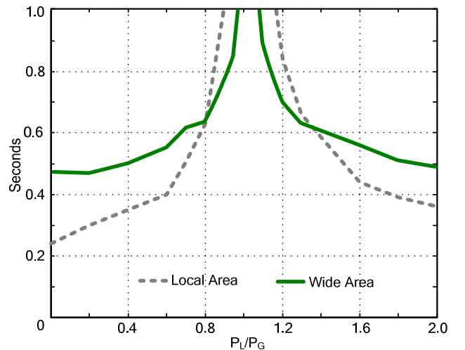
Fig. 11. Wide-Area Scheme Detects Islanding for All Power Exchange Conditions
