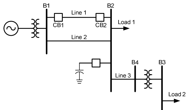
Fig. 15. Power System Model to Analyze RECIPE Technology in Real Time
