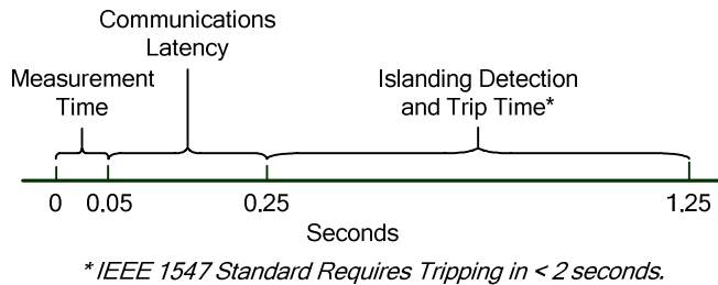
Fig. 12. Total Time to Detect Islanding and Trip Is 1.25 Seconds Using a Synchrophasor Wide-Area Measurement Scheme
