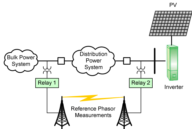
Fig. 9. Anti-Islanding Scheme Using an Inverter
