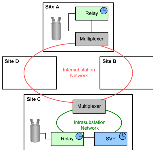
Fig. 3. Synchrophasor-Based Inter- and Intra-substation Networks
