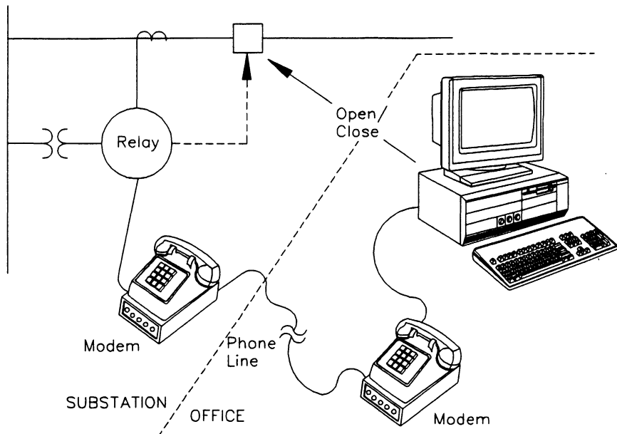
Figure 17: Control the Power-System Breaker Through Relay Commands
