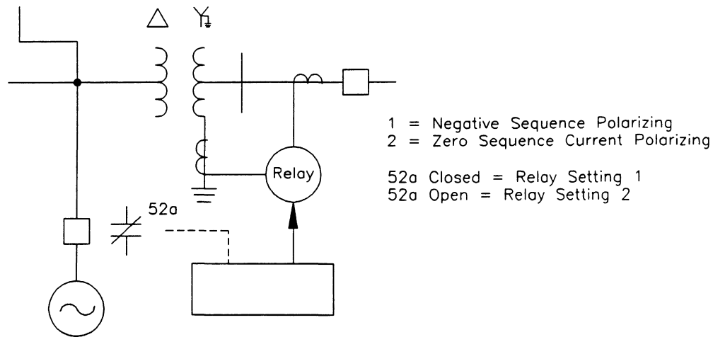
Figure 15: Change Relay Settings Based on Source Conditions
