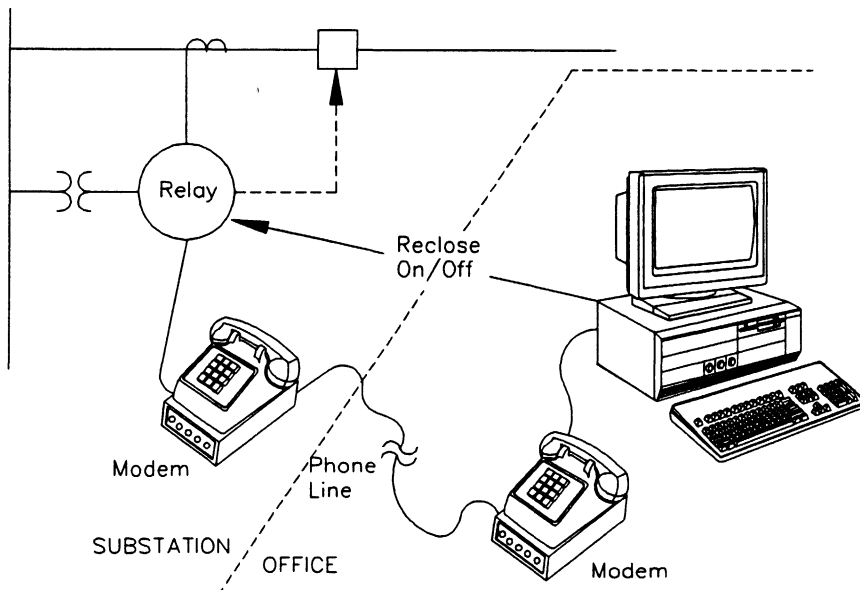
Figure 18: Remotely Control Auto-Reclosing
