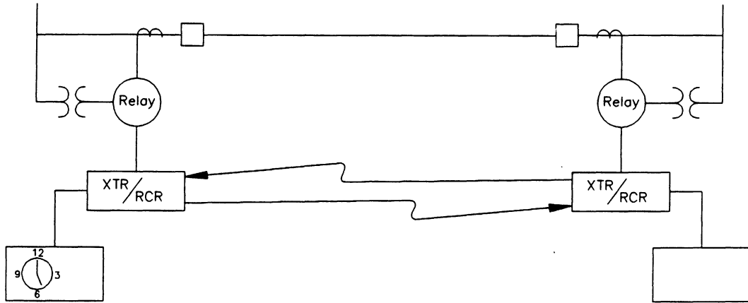
Figure 25: Automatically Check Pilot Scheme Communication
