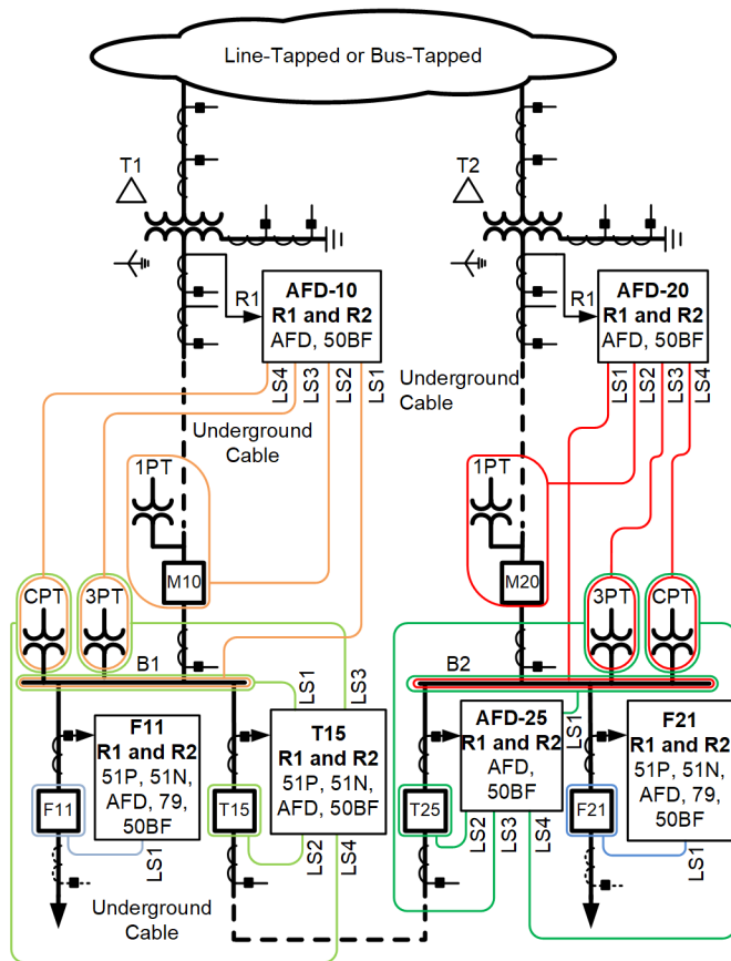
Fig. 5. Arc-flash protection scheme. Only one feeder per bus is shown for simplicity.
