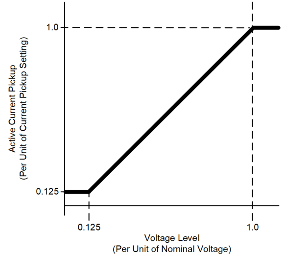
Fig. 11. Generic 51VR operating characteristics.
