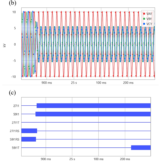
Fig. 8. Current (a) and voltage (b) waveforms for the fault and the IED response (c).
