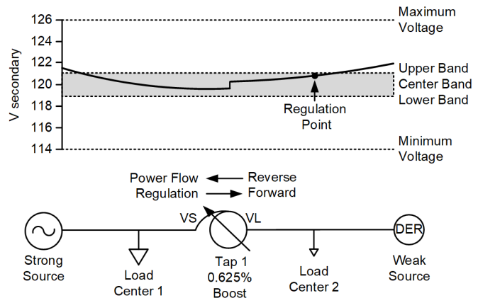
Fig. 16. Voltage regulation under reverse power during DER export.
