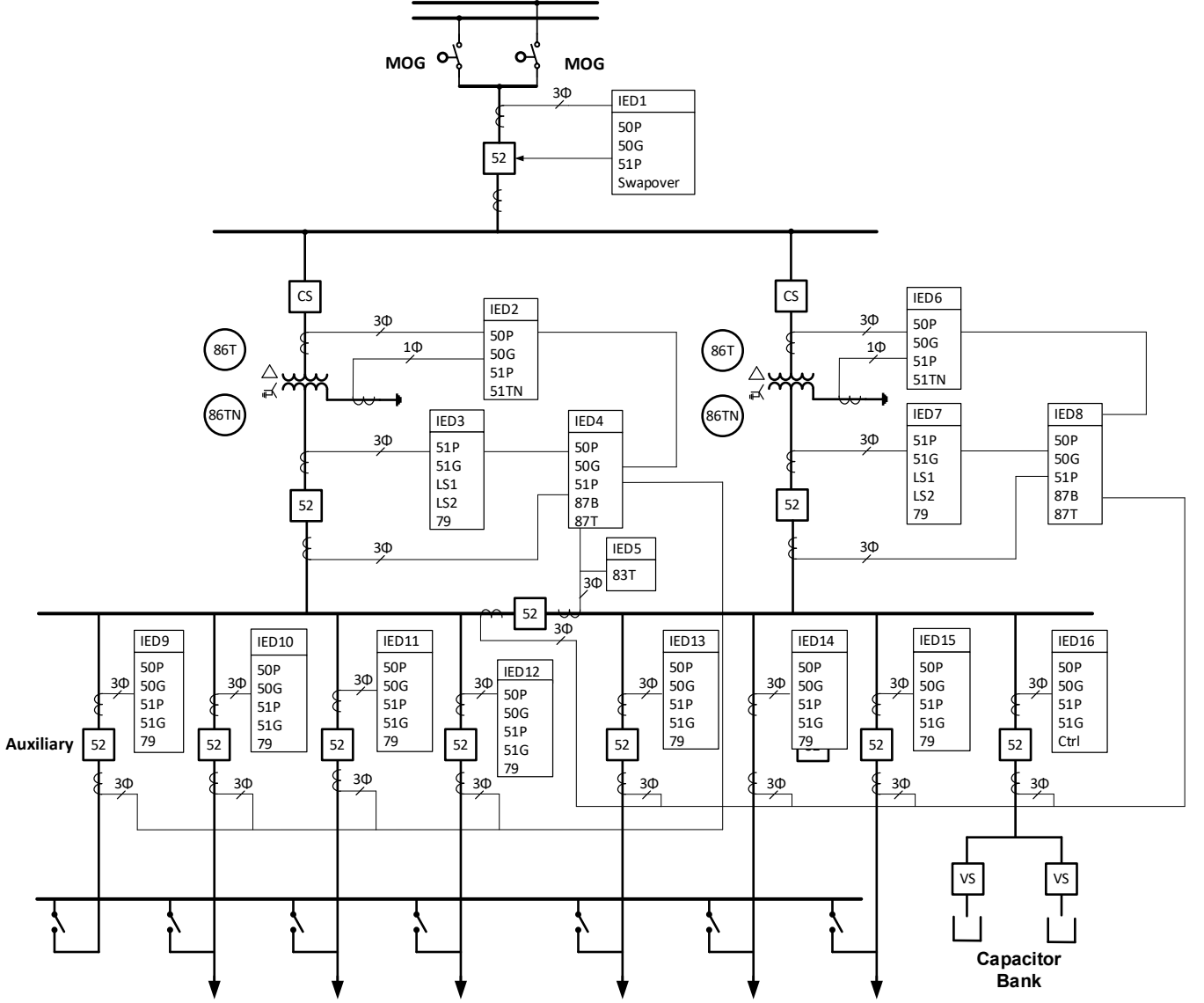
Fig. 2. Two-transformer distribution substation with bus tie breaker, auxiliary breaker, capacitor, and high-side swapover.
