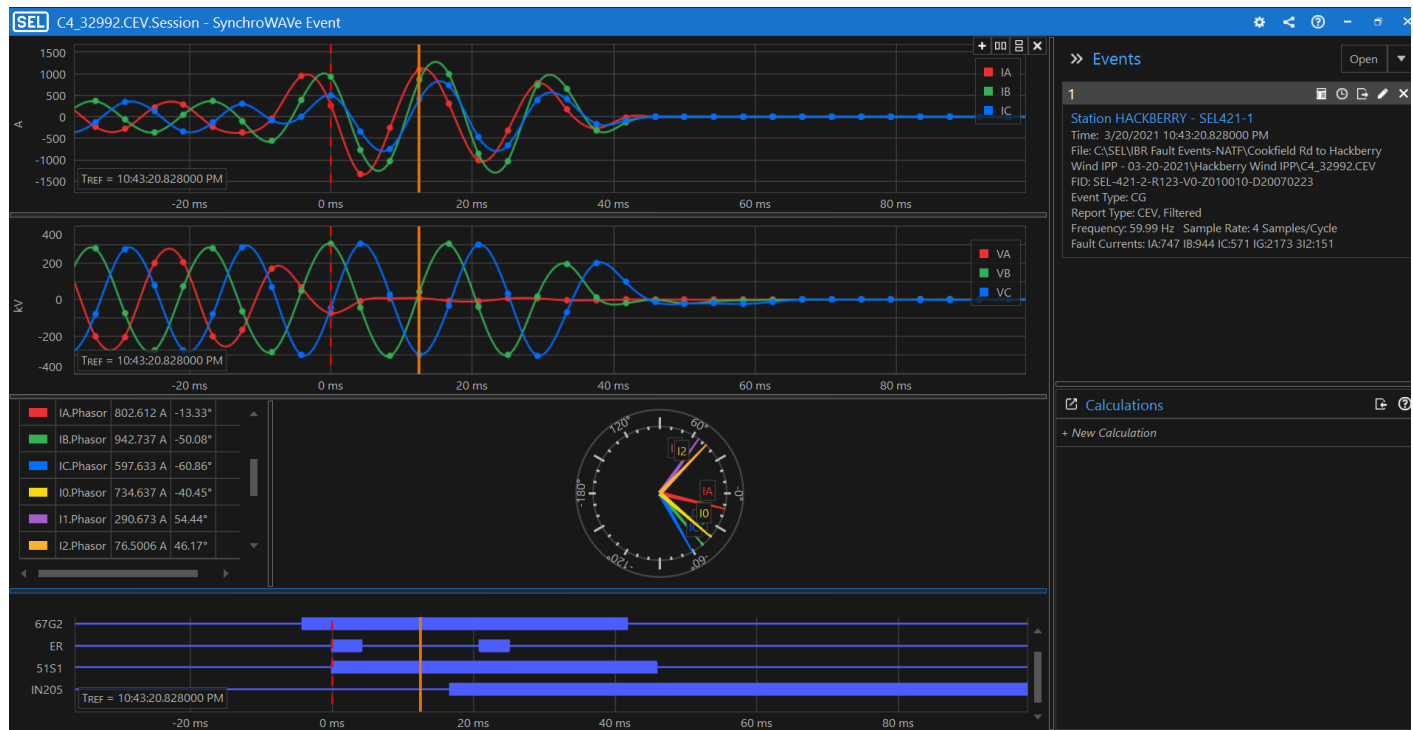
Figure 8. Oscillography from event recording relay near IBR
